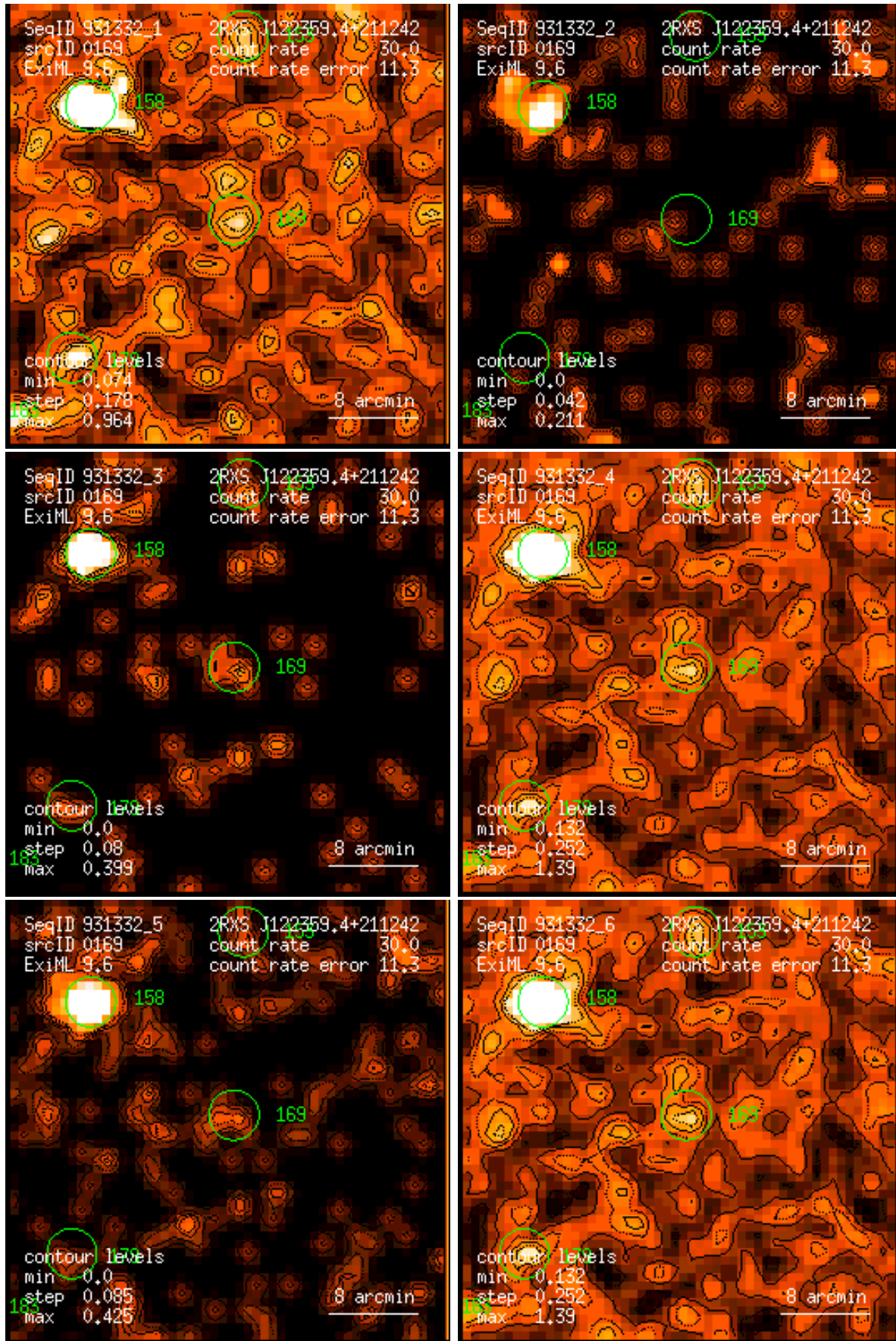
Figure 169: RASS 931332: detection 0169: band rate images, Gaussian filter: (1) PSPC channels 11 – 41, (2) 52 – 90, (3) 91 – 201, (4) 11 – 235, (5) 52 – 201, (6) 11 – 201. Broad band rates in counts/ks. Band rate contour levels in counts/ks/arcmin 2 .
