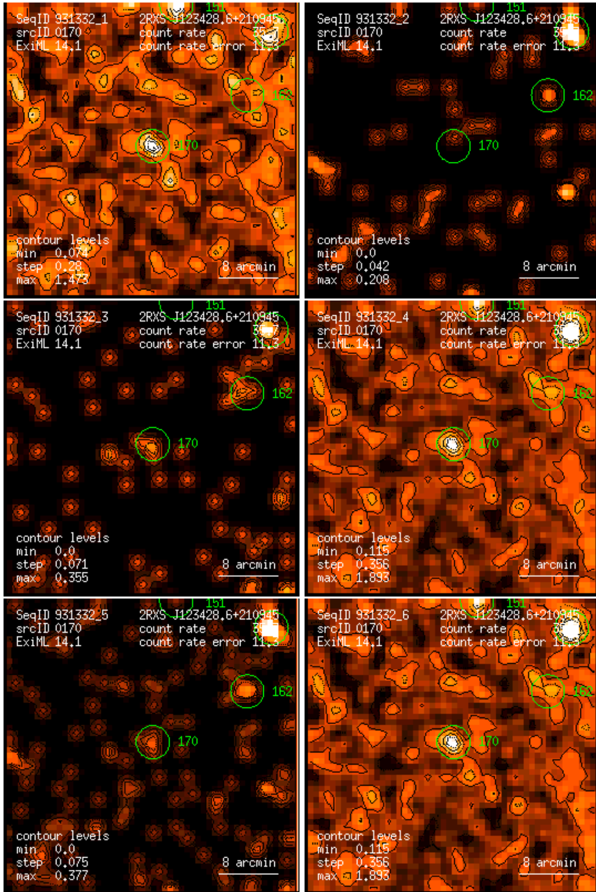
Figure 170: RASS 931332: detection 0170: band rate images, Gaussian filter: (1) PSPC channels 11 – 41, (2) 52 – 90, (3) 91 – 201, (4) 11 – 235, (5) 52 – 201, (6) 11 – 201. Broad band rates in counts/ks. Band rate contour levels in counts/ks/arcmin 2 .
