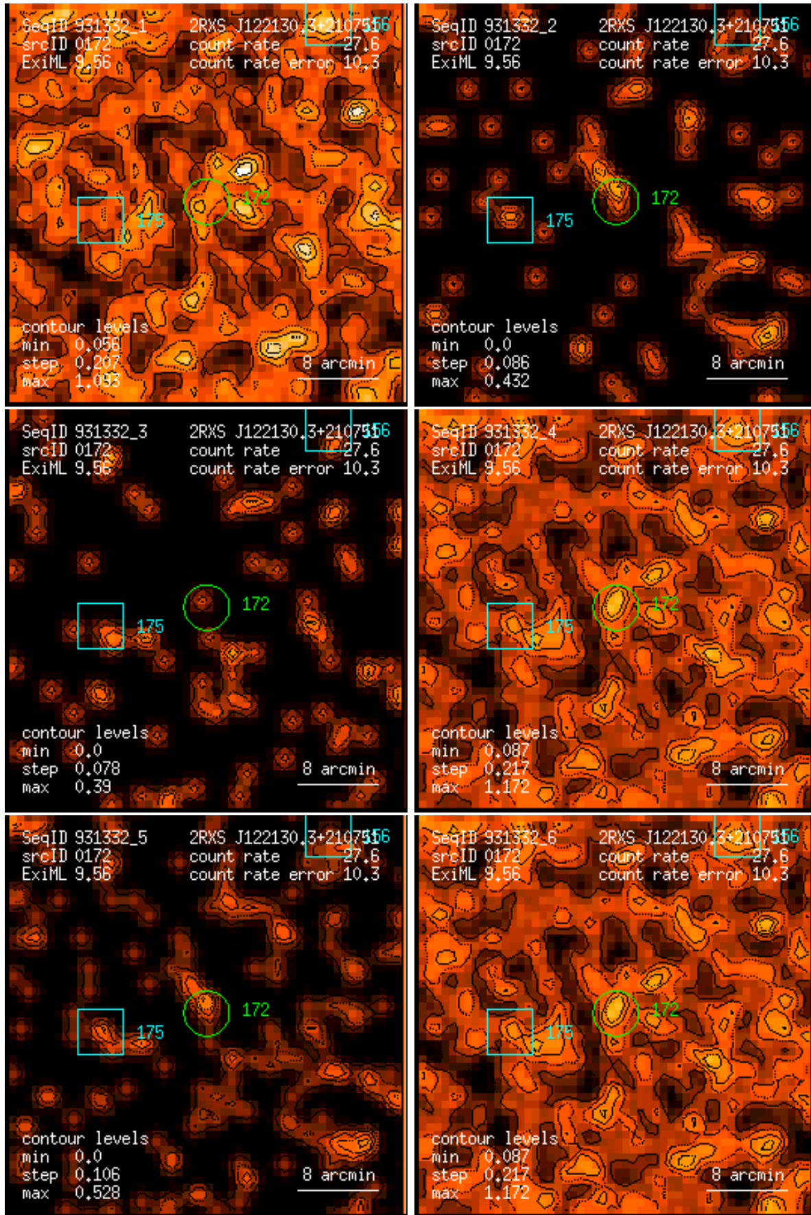
Figure 172: RASS 931332: detection 0172: band rate images, Gaussian filter: (1) PSPC channels 11 – 41, (2) 52 – 90, (3) 91 – 201, (4) 11 – 235, (5) 52 – 201, (6) 11 – 201. Broad band rates in counts/ks. Band rate contour levels in counts/ks/arcmin 2 .
