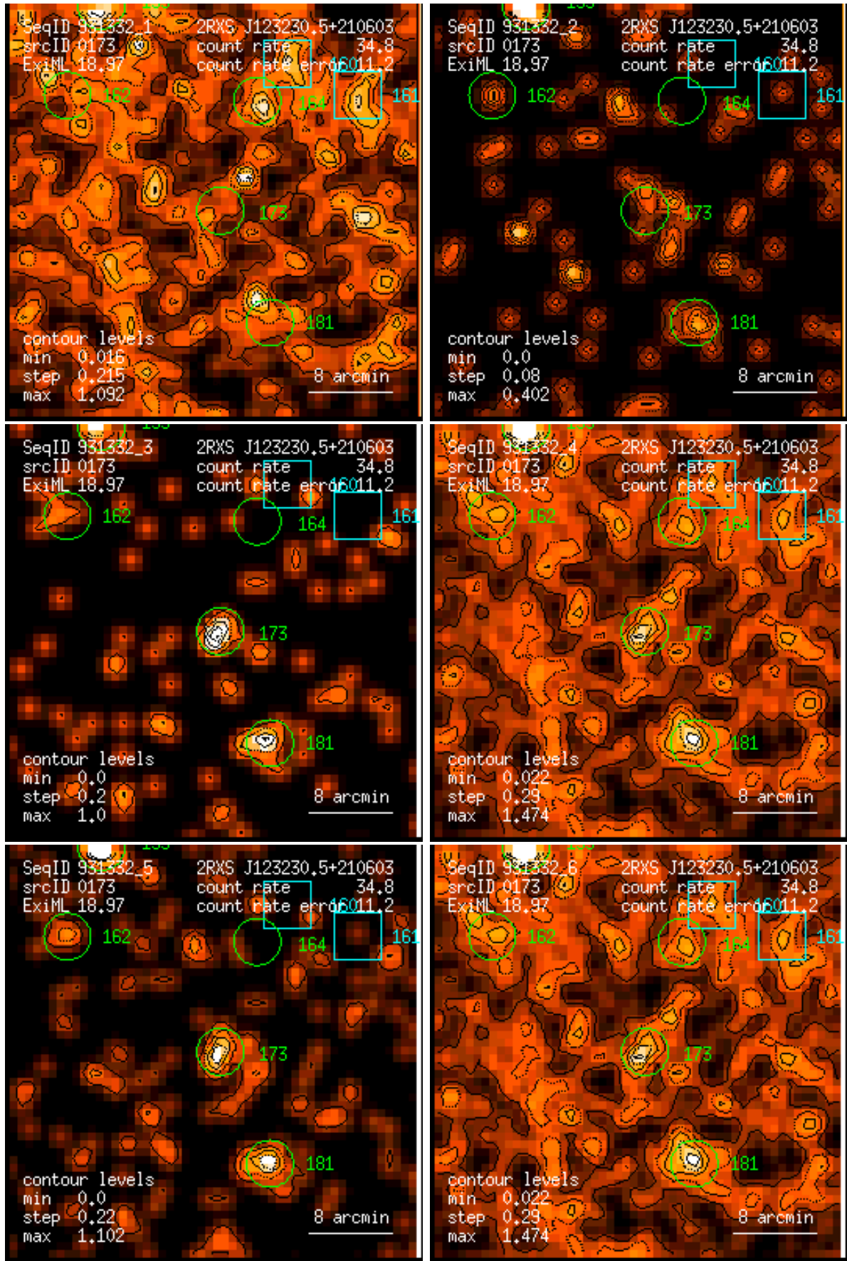
Figure 173: RASS 931332: detection 0173: band rate images, Gaussian filter: (1) PSPC channels 11 – 41, (2) 52 – 90, (3) 91 – 201, (4) 11 – 235, (5) 52 – 201, (6) 11 – 201. Broad band rates in counts/ks. Band rate contour levels in counts/ks/arcmin 2 .
