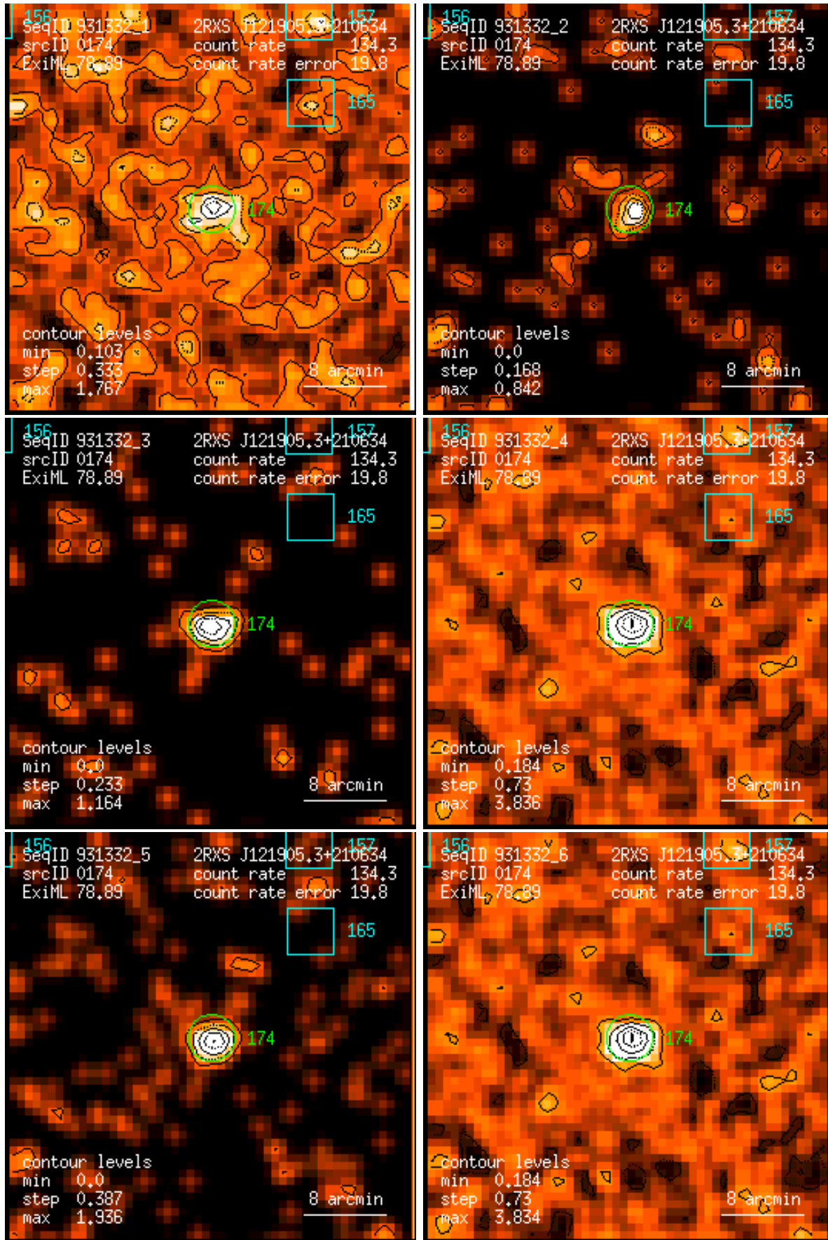
Figure 174: RASS 931332: detection 0174: band rate images, Gaussian filter: (1) PSPC channels 11 – 41, (2) 52 – 90, (3) 91 – 201, (4) 11 – 235, (5) 52 – 201, (6) 11 – 201. Broad band rates in counts/ks. Band rate contour levels in counts/ks/arcmin 2 .
