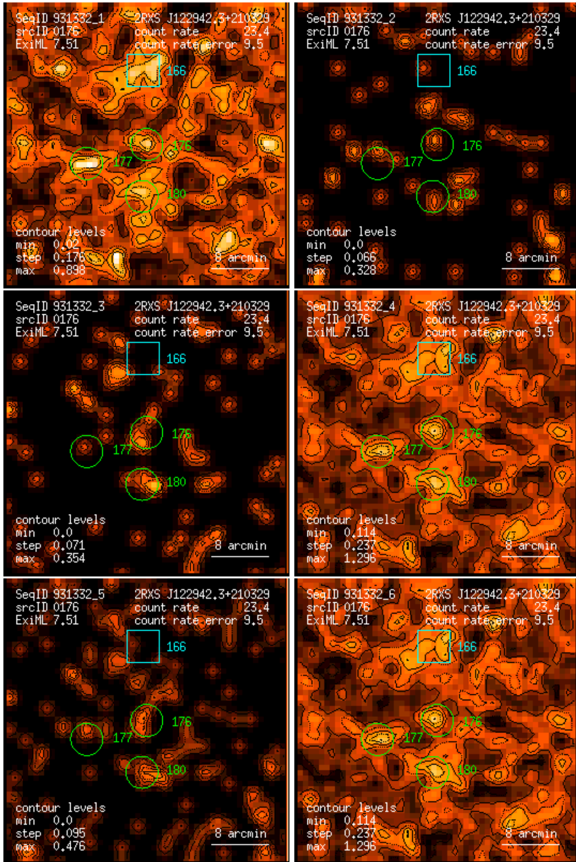
Figure 176: RASS 931332: detection 0176: band rate images, Gaussian filter: (1) PSPC channels 11 – 41, (2) 52 – 90, (3) 91 – 201, (4) 11 – 235, (5) 52 – 201, (6) 11 – 201. Broad band rates in counts/ks. Band rate contour levels in counts/ks/arcmin 2 .
