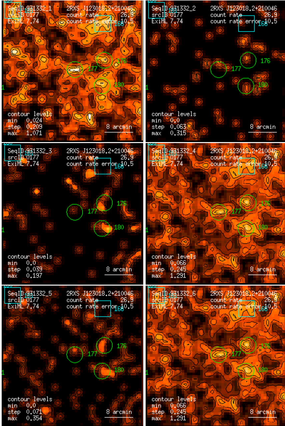
Figure 177: RASS 931332: detection 0177: band rate images, Gaussian filter: (1) PSPC channels 11 – 41, (2) 52 – 90, (3) 91 – 201, (4) 11 – 235, (5) 52 – 201, (6) 11 – 201. Broad band rates in counts/ks. Band rate contour levels in counts/ks/arcmin 2 .
