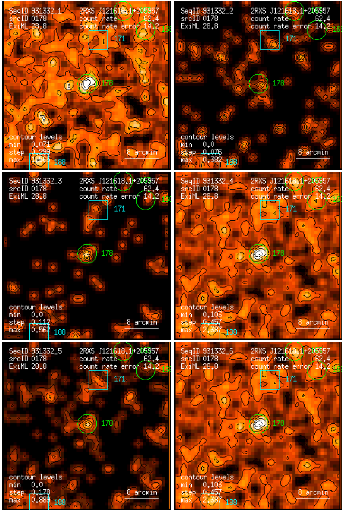
Figure 178: RASS 931332: detection 0178: band rate images, Gaussian filter: (1) PSPC channels 11 – 41, (2) 52 – 90, (3) 91 – 201, (4) 11 – 235, (5) 52 – 201, (6) 11 – 201. Broad band rates in counts/ks. Band rate contour levels in counts/ks/arcmin 2 .
