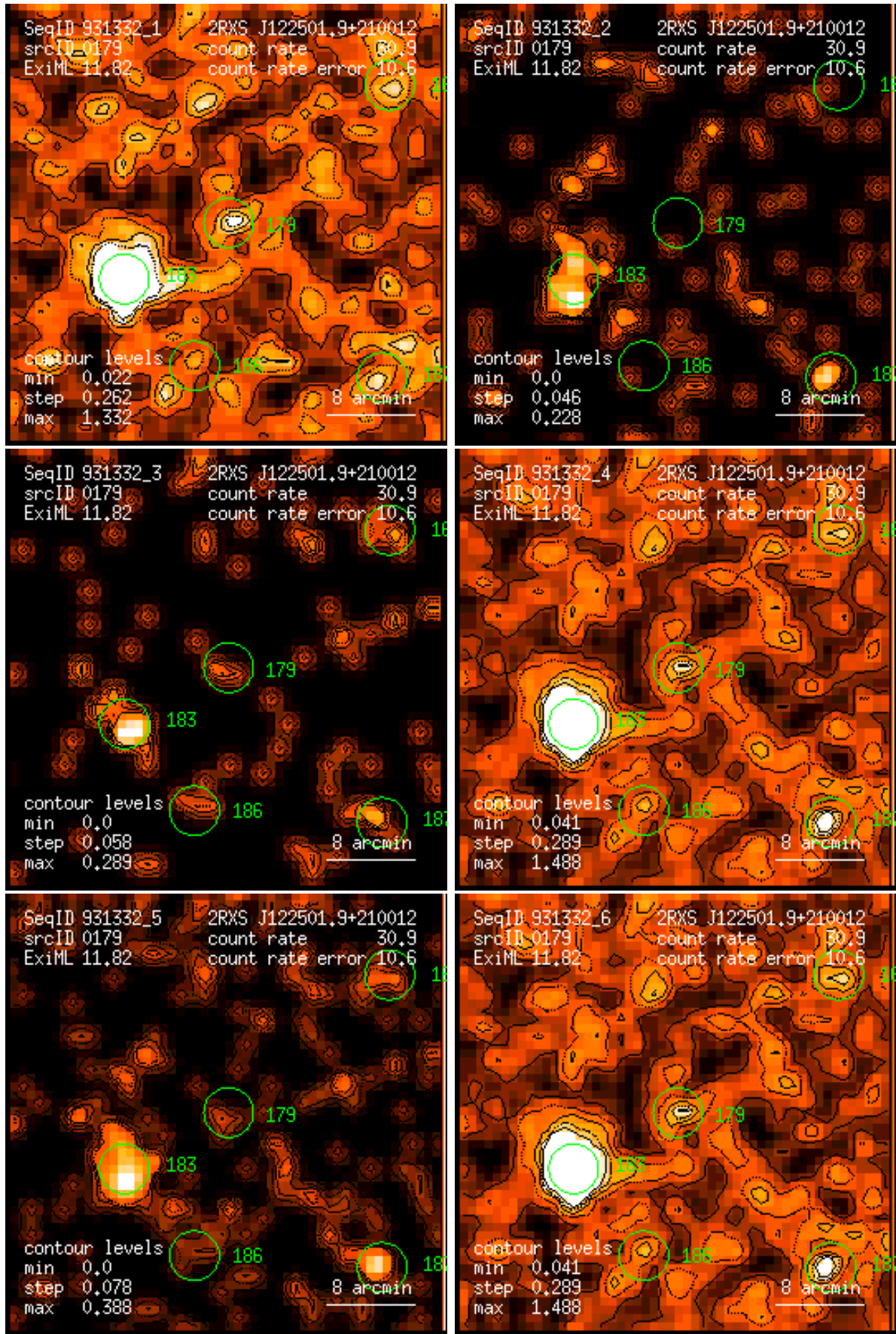
Figure 179: RASS 931332: detection 0179: band rate images, Gaussian filter: (1) PSPC channels 11 – 41, (2) 52 – 90, (3) 91 – 201, (4) 11 – 235, (5) 52 – 201, (6) 11 – 201. Broad band rates in counts/ks. Band rate contour levels in counts/ks/arcmin 2 .
