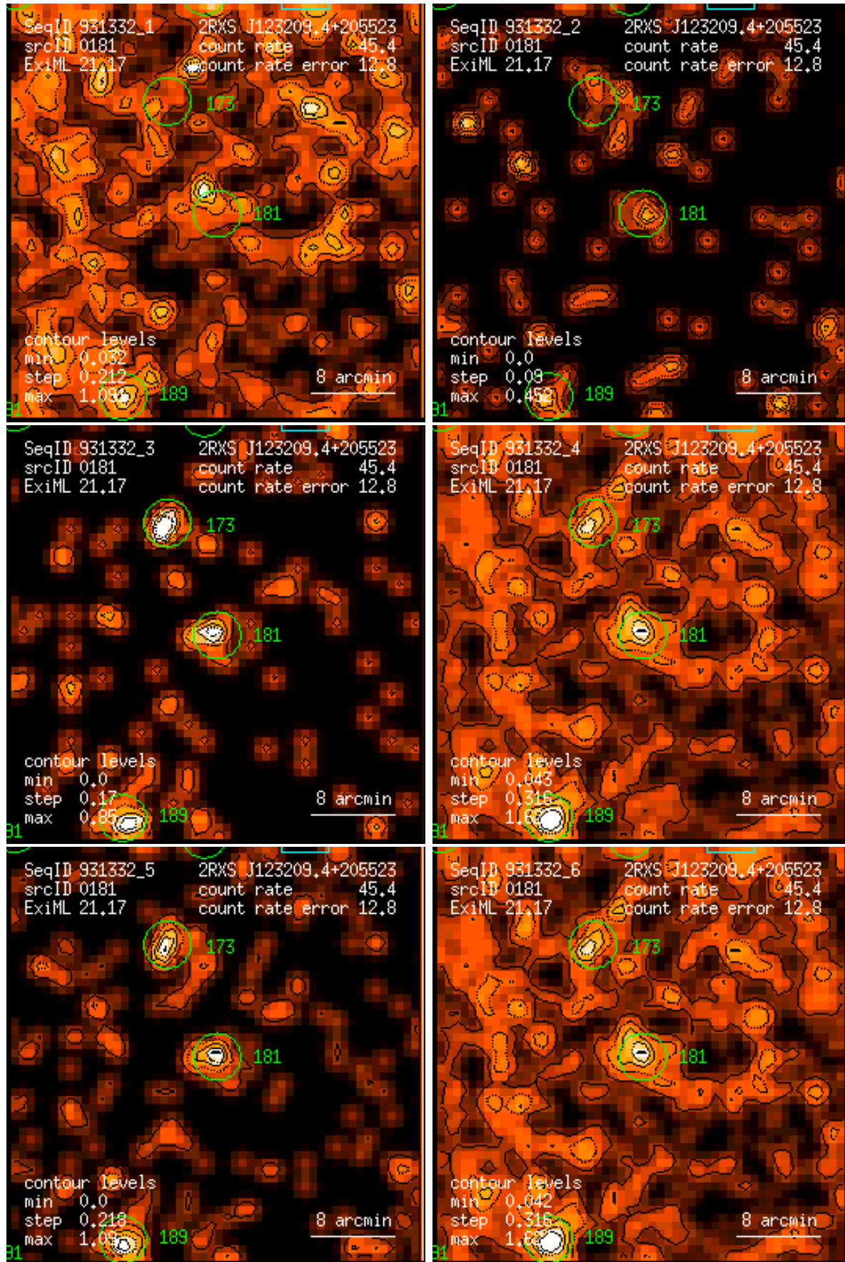
Figure 181: RASS 931332: detection 0181: band rate images, Gaussian filter: (1) PSPC channels 11 – 41, (2) 52 – 90, (3) 91 – 201, (4) 11 – 235, (5) 52 – 201, (6) 11 – 201. Broad band rates in counts/ks. Band rate contour levels in counts/ks/arcmin 2 .
