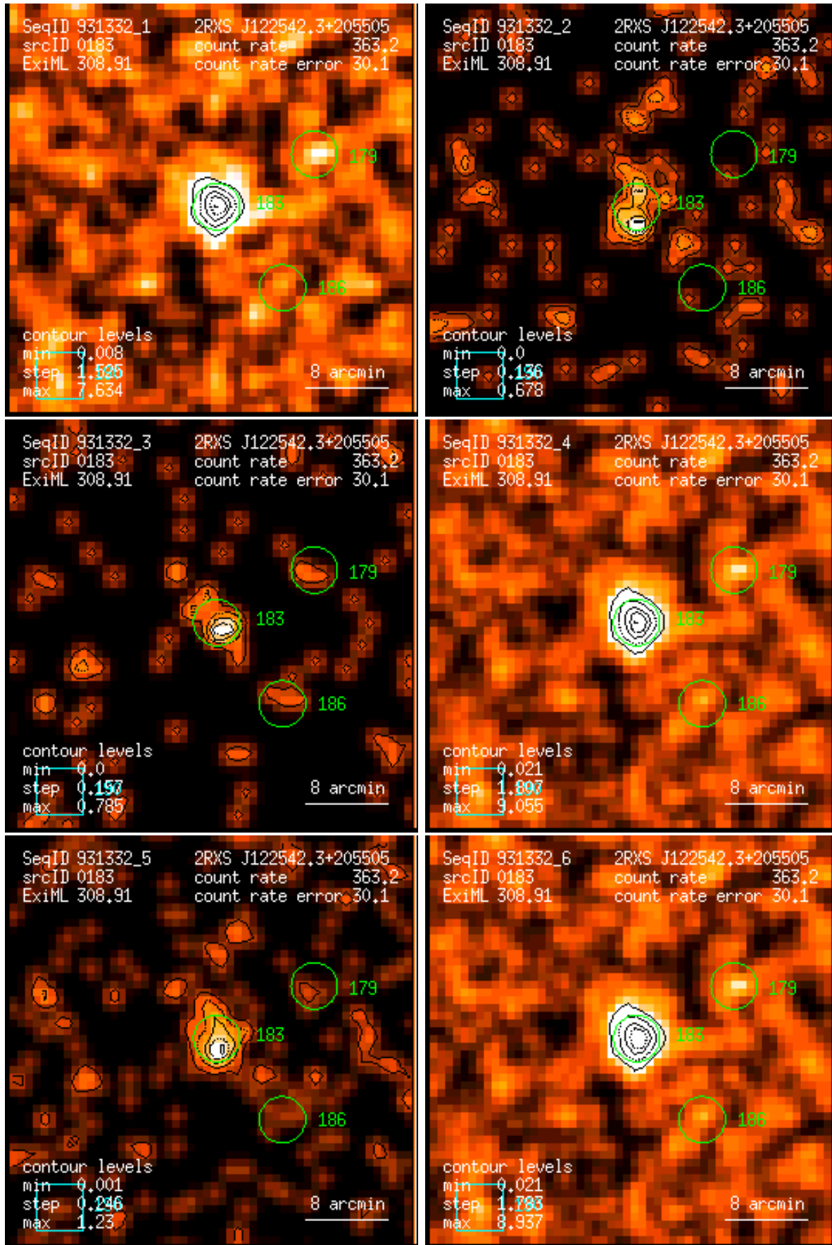
Figure 183: RASS 931332: detection 0183: band rate images, Gaussian filter: (1) PSPC channels 11 – 41, (2) 52 – 90, (3) 91 – 201, (4) 11 – 235, (5) 52 – 201, (6) 11 – 201. Broad band rates in counts/ks. Band rate contour levels in counts/ks/arcmin 2 .
