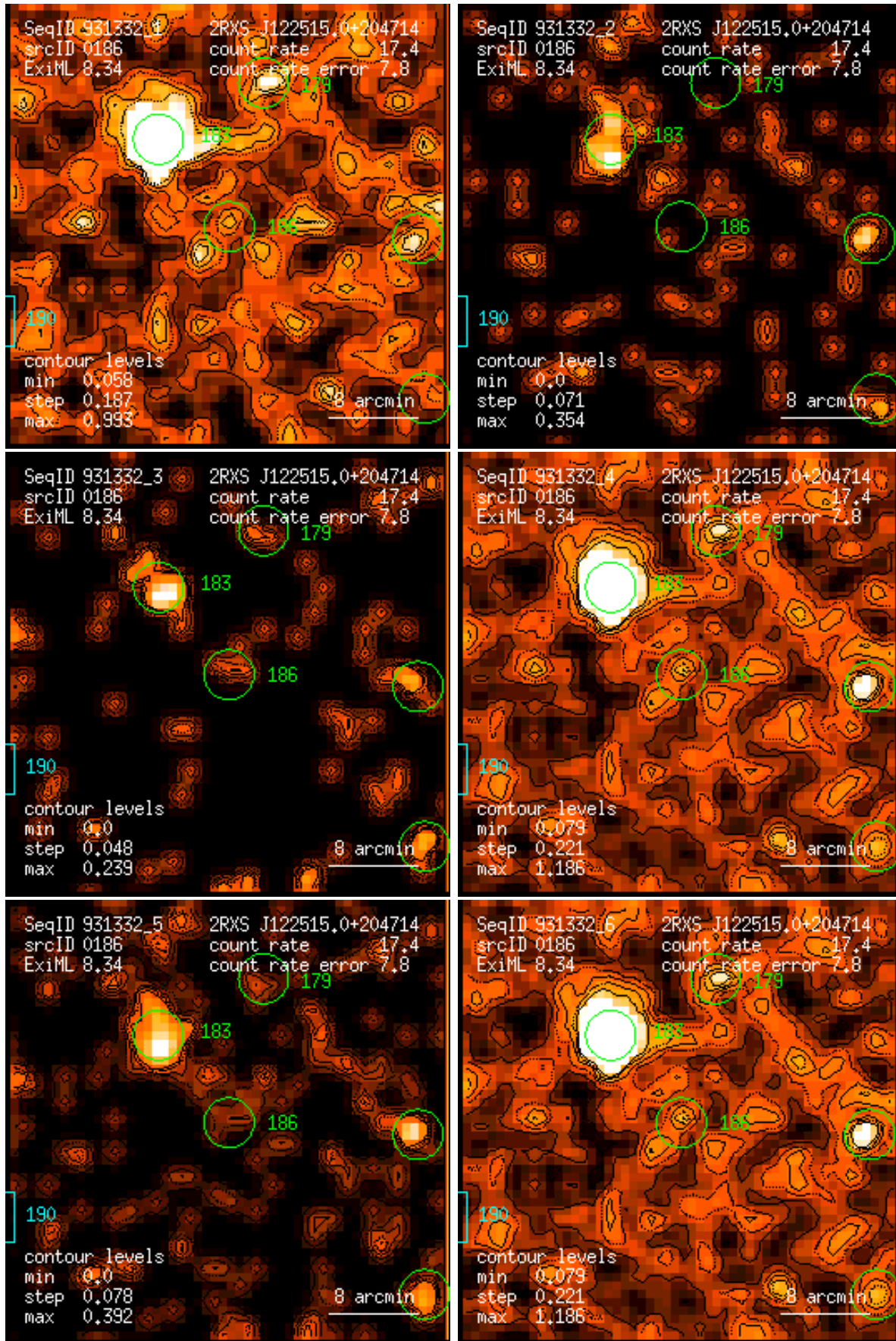
Figure 186: RASS 931332: detection 0186: band rate images, Gaussian filter: (1) PSPC channels 11 – 41, (2) 52 – 90, (3) 91 – 201, (4) 11 – 235, (5) 52 – 201, (6) 11 – 201. Broad band rates in counts/ks. Band rate contour levels in counts/ks/arcmin 2 .
