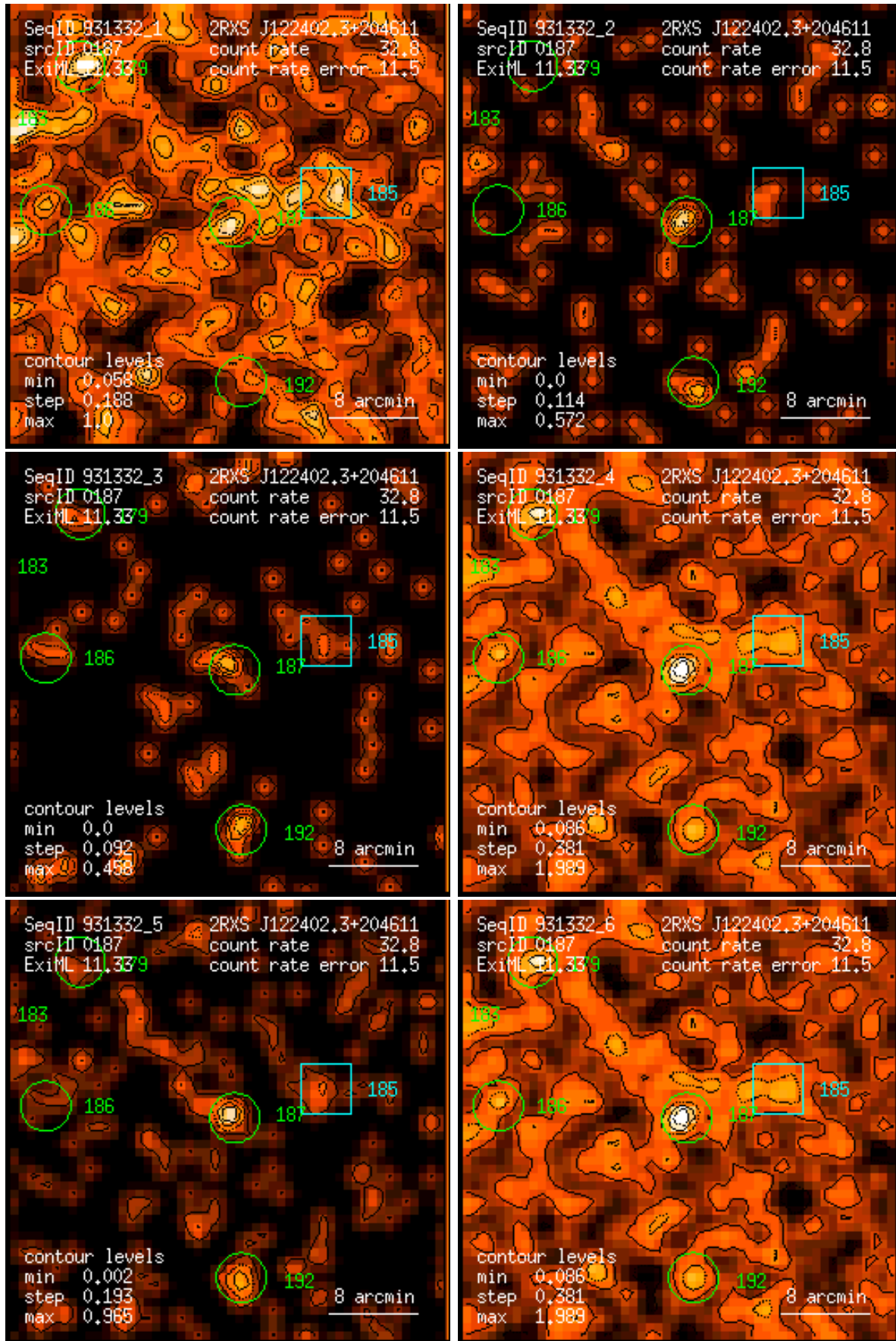
Figure 187: RASS 931332: detection 0187: band rate images, Gaussian filter: (1) PSPC channels 11 – 41, (2) 52 – 90, (3) 91 – 201, (4) 11 – 235, (5) 52 – 201, (6) 11 – 201. Broad band rates in counts/ks. Band rate contour levels in counts/ks/arcmin 2 .
