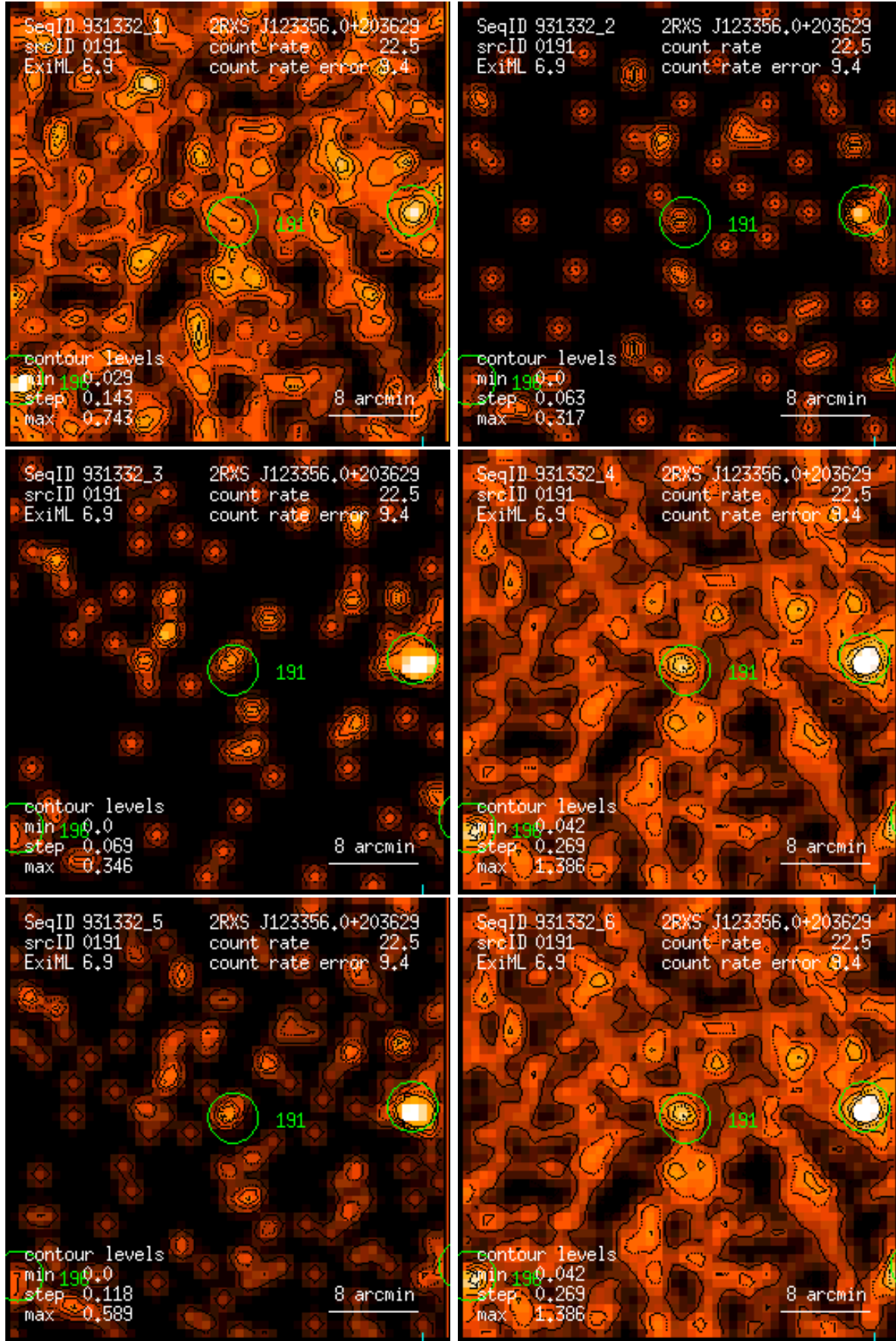
Figure 191: RASS 931332: detection 0191: band rate images, Gaussian filter: (1) PSPC channels 11 – 41, (2) 52 – 90, (3) 91 – 201, (4) 11 – 235, (5) 52 – 201, (6) 11 – 201. Broad band rates in counts/ks. Band rate contour levels in counts/ks/arcmin 2 .
