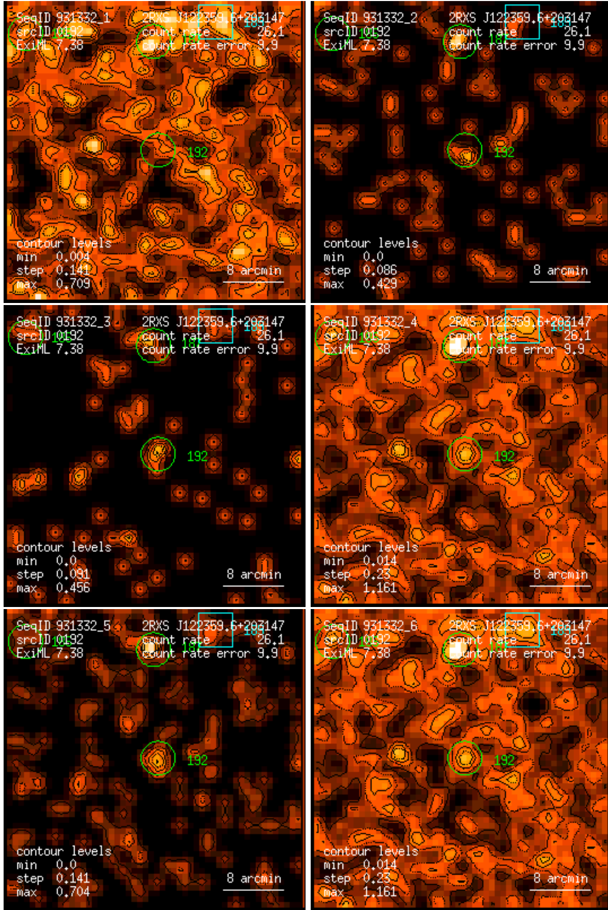
Figure 192: RASS 931332: detection 0192: band rate images, Gaussian filter: (1) PSPC channels 11 – 41, (2) 52 – 90, (3) 91 – 201, (4) 11 – 235, (5) 52 – 201, (6) 11 – 201. Broad band rates in counts/ks. Band rate contour levels in counts/ks/arcmin 2 .
