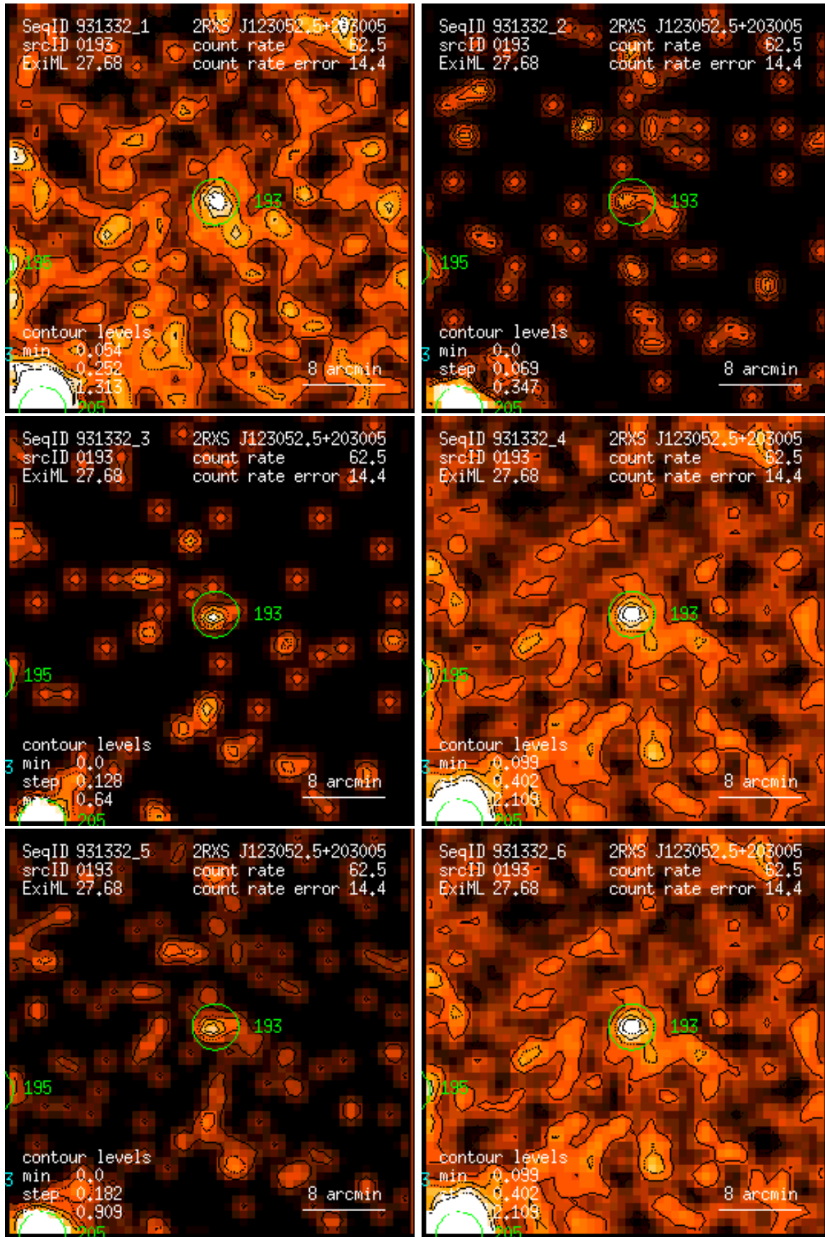
Figure 193: RASS 931332: detection 0193: band rate images, Gaussian filter: (1) PSPC channels 11 – 41, (2) 52 – 90, (3) 91 – 201, (4) 11 – 235, (5) 52 – 201, (6) 11 – 201. Broad band rates in counts/ks. Band rate contour levels in counts/ks/arcmin 2 .
