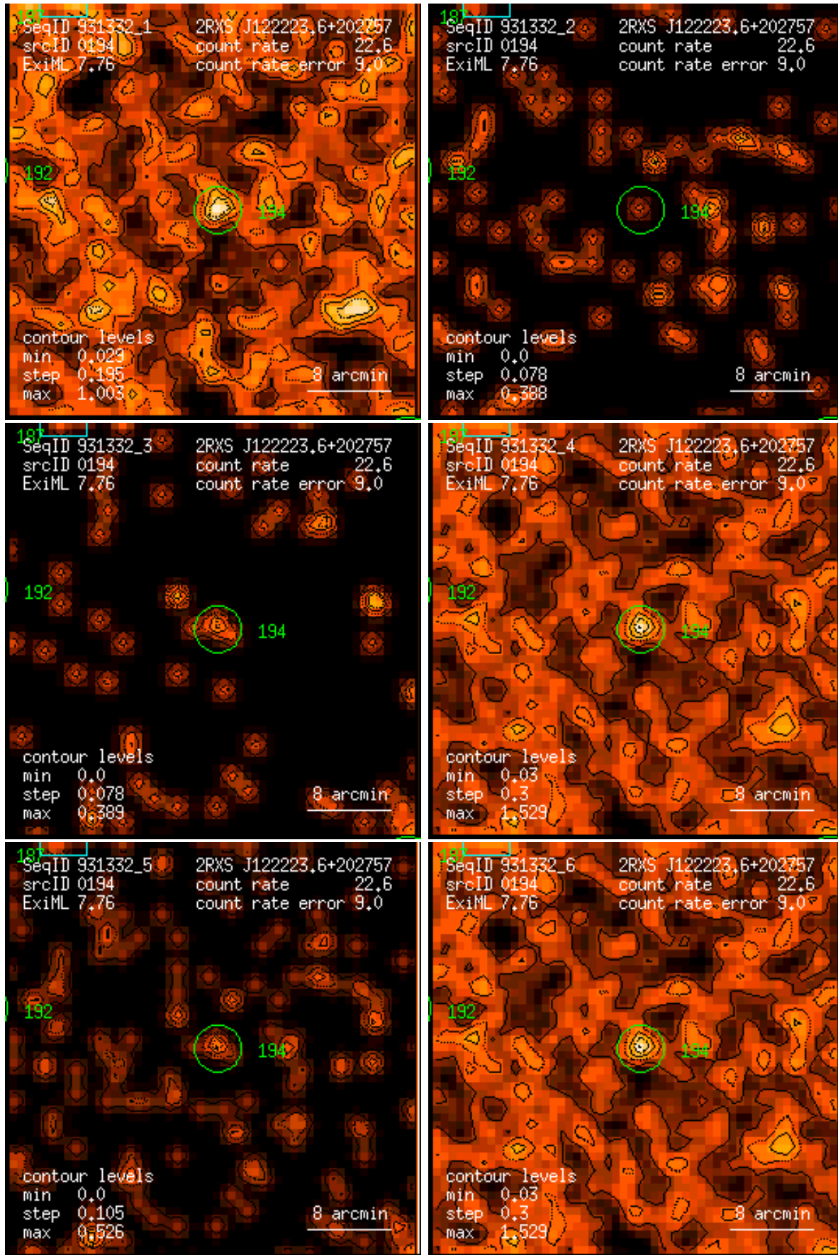
Figure 194: RASS 931332: detection 0194: band rate images, Gaussian filter: (1) PSPC channels 11 – 41, (2) 52 – 90, (3) 91 – 201, (4) 11 – 235, (5) 52 – 201, (6) 11 – 201. Broad band rates in counts/ks. Band rate contour levels in counts/ks/arcmin 2 .
