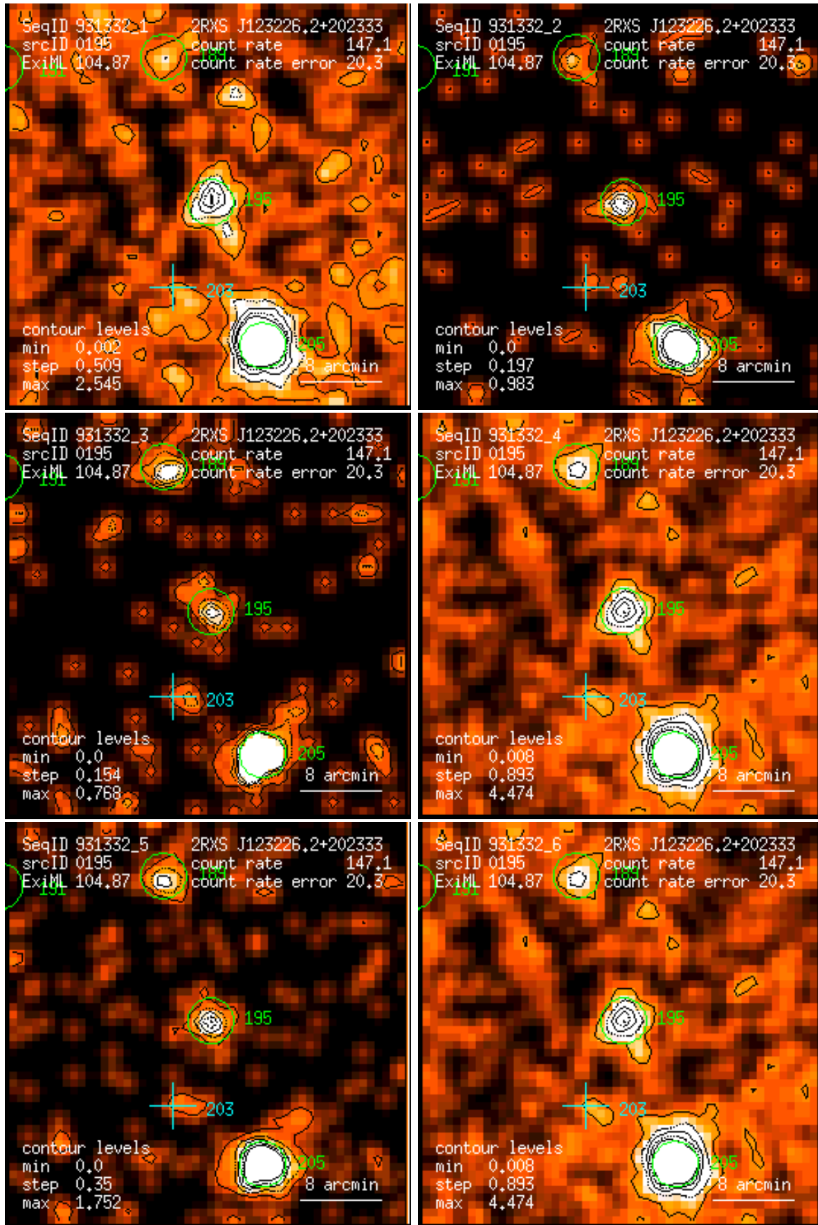
Figure 195: RASS 931332: detection 0195: band rate images, Gaussian filter: (1) PSPC channels 11 – 41, (2) 52 – 90, (3) 91 – 201, (4) 11 – 235, (5) 52 – 201, (6) 11 – 201. Broad band rates in counts/ks. Band rate contour levels in counts/ks/arcmin 2 .
