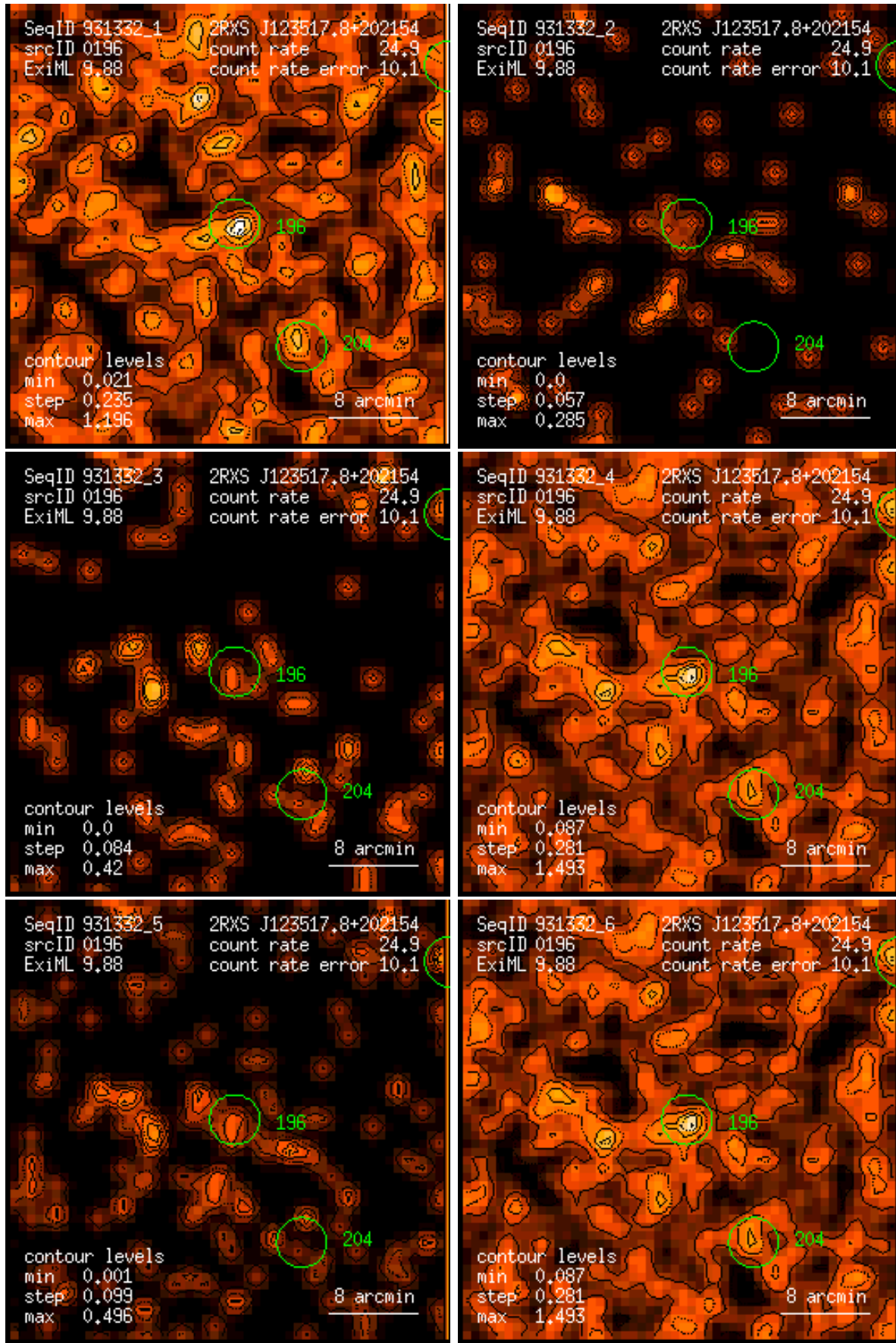
Figure 196: RASS 931332: detection 0196: band rate images, Gaussian filter: (1) PSPC channels 11 – 41, (2) 52 – 90, (3) 91 – 201, (4) 11 – 235, (5) 52 – 201, (6) 11 – 201. Broad band rates in counts/ks. Band rate contour levels in counts/ks/arcmin 2 .
