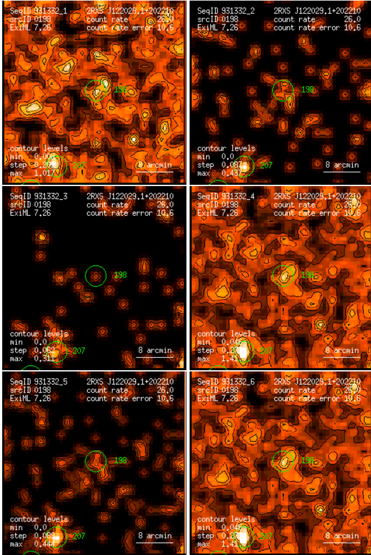
Figure 198: RASS 931332: detection 0198: band rate images, Gaussian filter: (1) PSPC channels 11 – 41, (2) 52 – 90, (3) 91 – 201, (4) 11 – 235, (5) 52 – 201, (6) 11 – 201. Broad band rates in counts/ks. Band rate contour levels in counts/ks/arcmin 2 .
