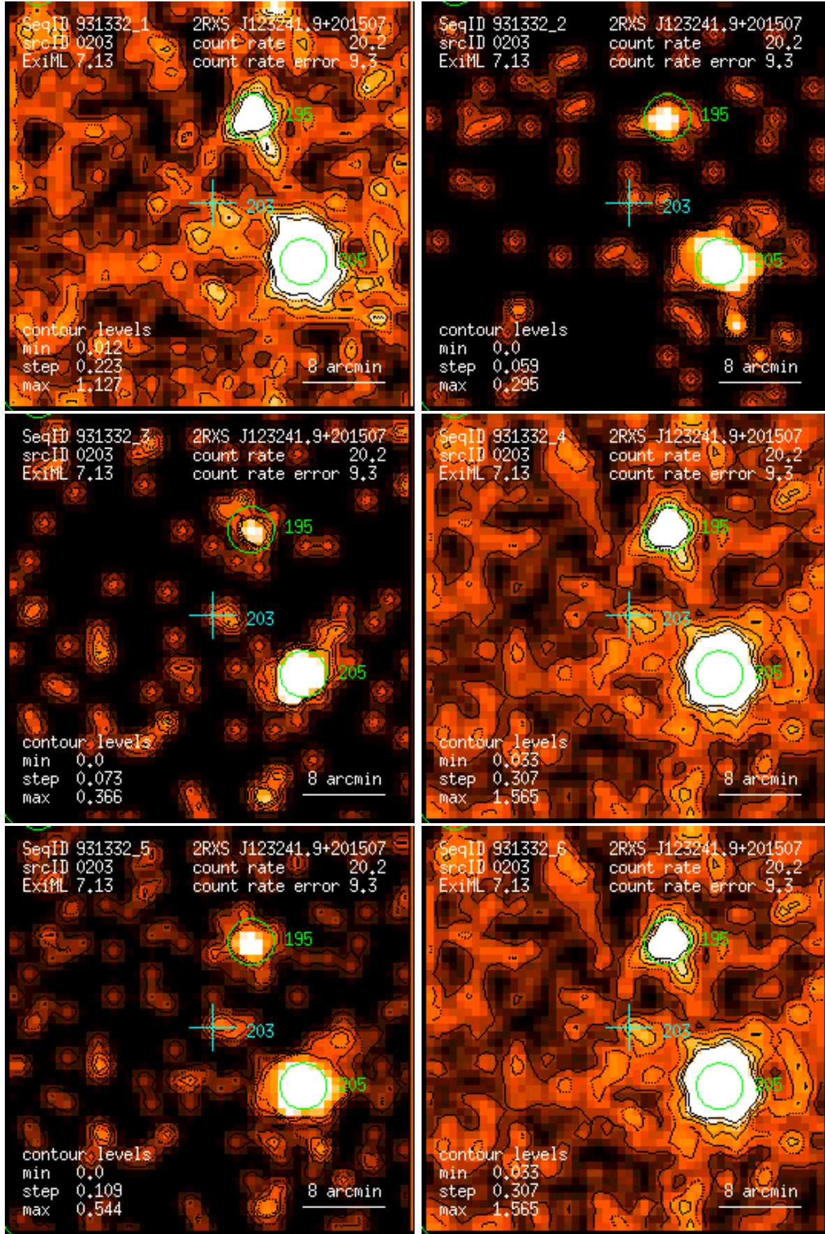
Figure 203: RASS 931332: detection 0203: band rate images, Gaussian filter: (1) PSPC channels 11 – 41, (2) 52 – 90, (3) 91 – 201, (4) 11 – 235, (5) 52 – 201, (6) 11 – 201. Broad band rates in counts/ks. Band rate contour levels in counts/ks/arcmin 2 .
