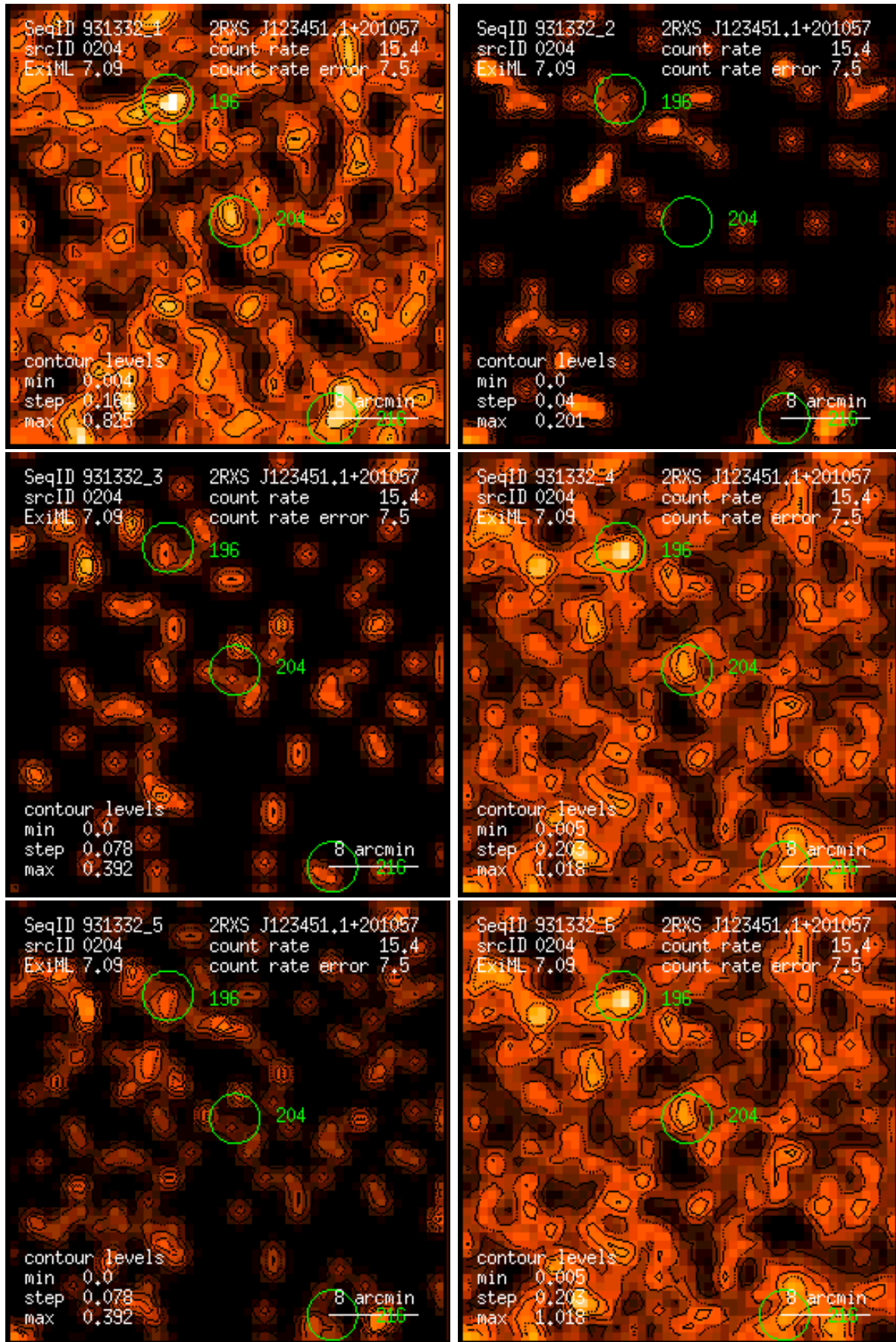
Figure 204: RASS 931332: detection 0204: band rate images, Gaussian filter: (1) PSPC channels 11 – 41, (2) 52 – 90, (3) 91 – 201, (4) 11 – 235, (5) 52 – 201, (6) 11 – 201. Broad band rates in counts/ks. Band rate contour levels in counts/ks/arcmin 2 .
