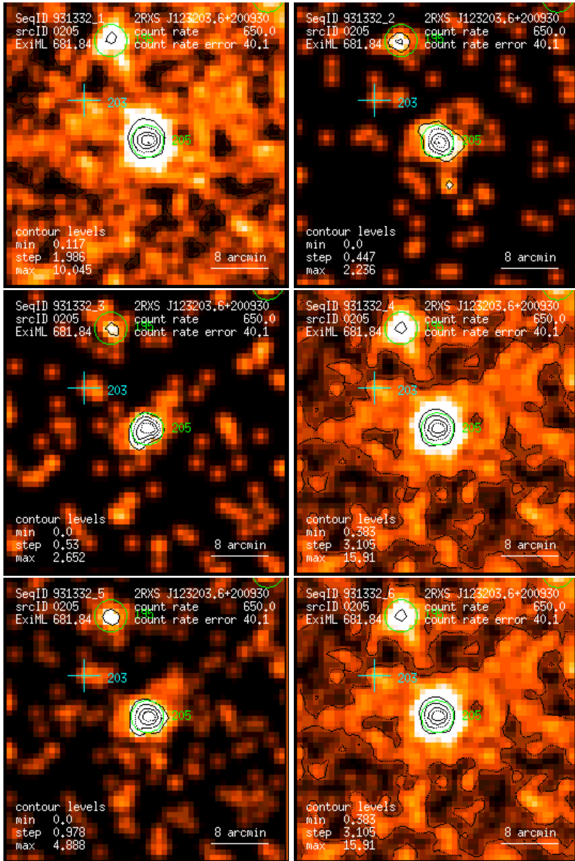
Figure 205: RASS 931332: detection 0205: band rate images, Gaussian filter: (1) PSPC channels 11 – 41, (2) 52 – 90, (3) 91 – 201, (4) 11 – 235, (5) 52 – 201, (6) 11 – 201. Broad band rates in counts/ks. Band rate contour levels in counts/ks/arcmin 2 .
