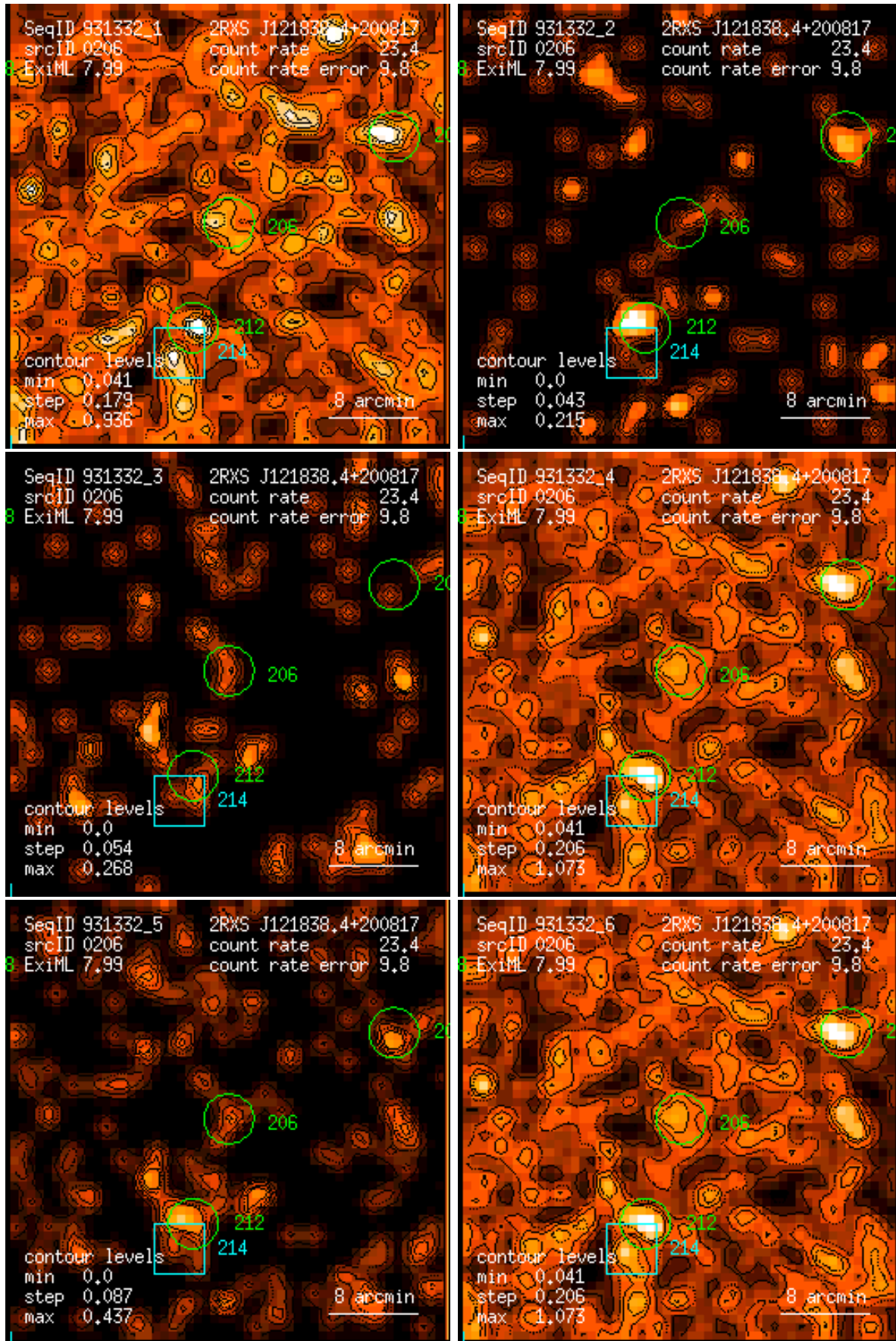
Figure 206: RASS 931332: detection 0206: band rate images, Gaussian filter: (1) PSPC channels 11 – 41, (2) 52 – 90, (3) 91 – 201, (4) 11 – 235, (5) 52 – 201, (6) 11 – 201. Broad band rates in counts/ks. Band rate contour levels in counts/ks/arcmin 2 .
