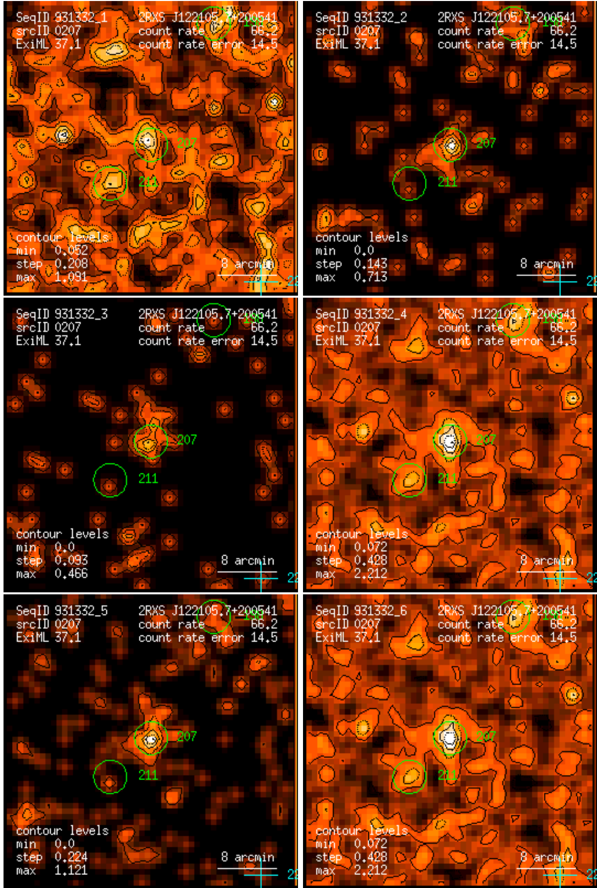
Figure 207: RASS 931332: detection 0207: band rate images, Gaussian filter: (1) PSPC channels 11 – 41, (2) 52 – 90, (3) 91 – 201, (4) 11 – 235, (5) 52 – 201, (6) 11 – 201. Broad band rates in counts/ks. Band rate contour levels in counts/ks/arcmin 2 .
