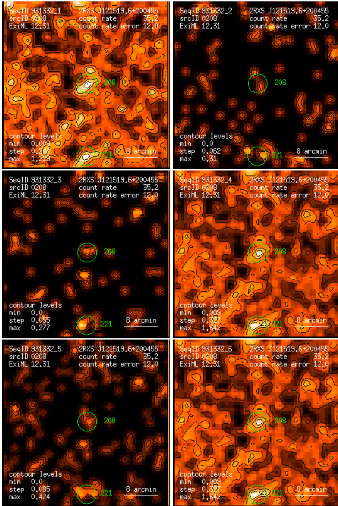
Figure 208: RASS 931332: detection 0208: band rate images, Gaussian filter: (1) PSPC channels 11 – 41, (2) 52 – 90, (3) 91 – 201, (4) 11 – 235, (5) 52 – 201, (6) 11 – 201. Broad band rates in counts/ks. Band rate contour levels in counts/ks/arcmin 2 .
