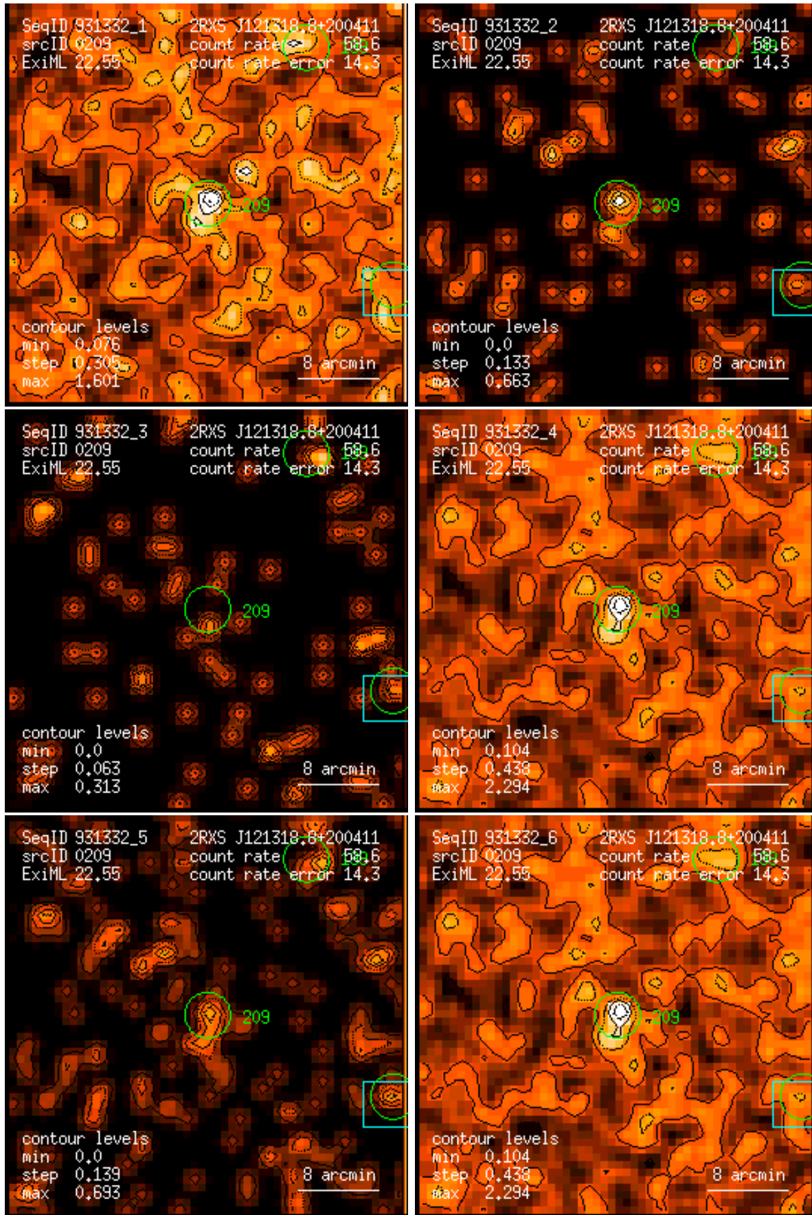
Figure 209: RASS 931332: detection 0209: band rate images, Gaussian filter: (1) PSPC channels 11 – 41, (2) 52 – 90, (3) 91 – 201, (4) 11 – 235, (5) 52 – 201, (6) 11 – 201. Broad band rates in counts/ks. Band rate contour levels in counts/ks/arcmin 2 .
