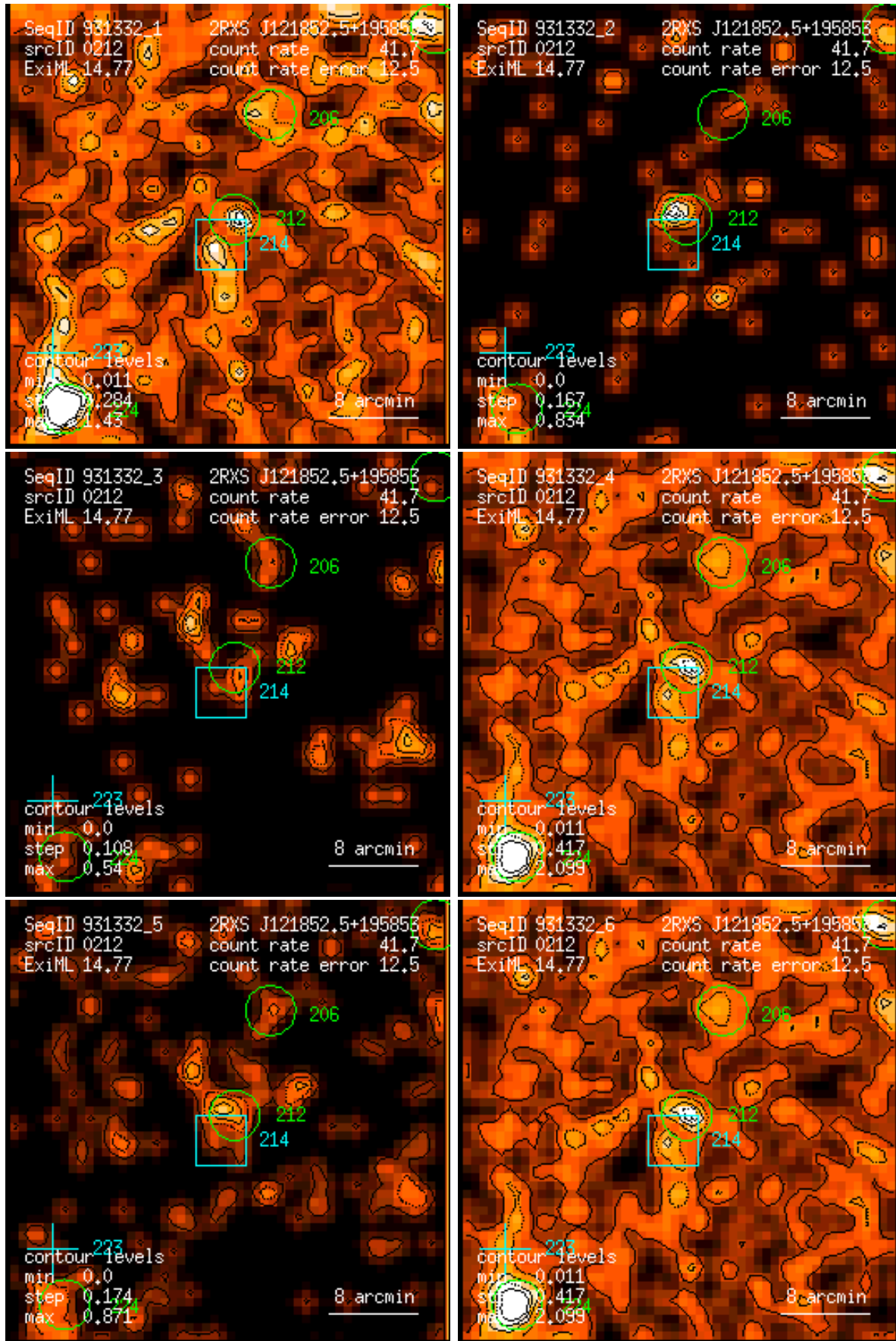
Figure 212: RASS 931332: detection 0212: band rate images, Gaussian filter: (1) PSPC channels 11 – 41, (2) 52 – 90, (3) 91 – 201, (4) 11 – 235, (5) 52 – 201, (6) 11 – 201. Broad band rates in counts/ks. Band rate contour levels in counts/ks/arcmin 2 .
