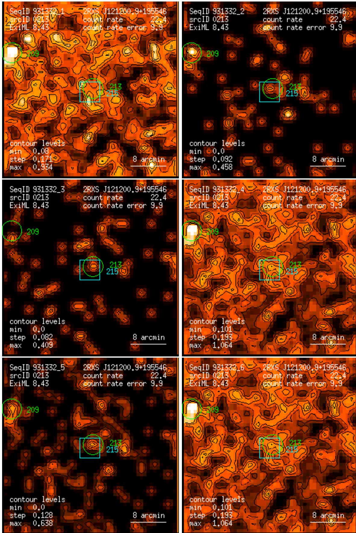
Figure 213: RASS 931332: detection 0213: band rate images, Gaussian filter: (1) PSPC channels 11 – 41, (2) 52 – 90, (3) 91 – 201, (4) 11 – 235, (5) 52 – 201, (6) 11 – 201. Broad band rates in counts/ks. Band rate contour levels in counts/ks/arcmin 2 .
