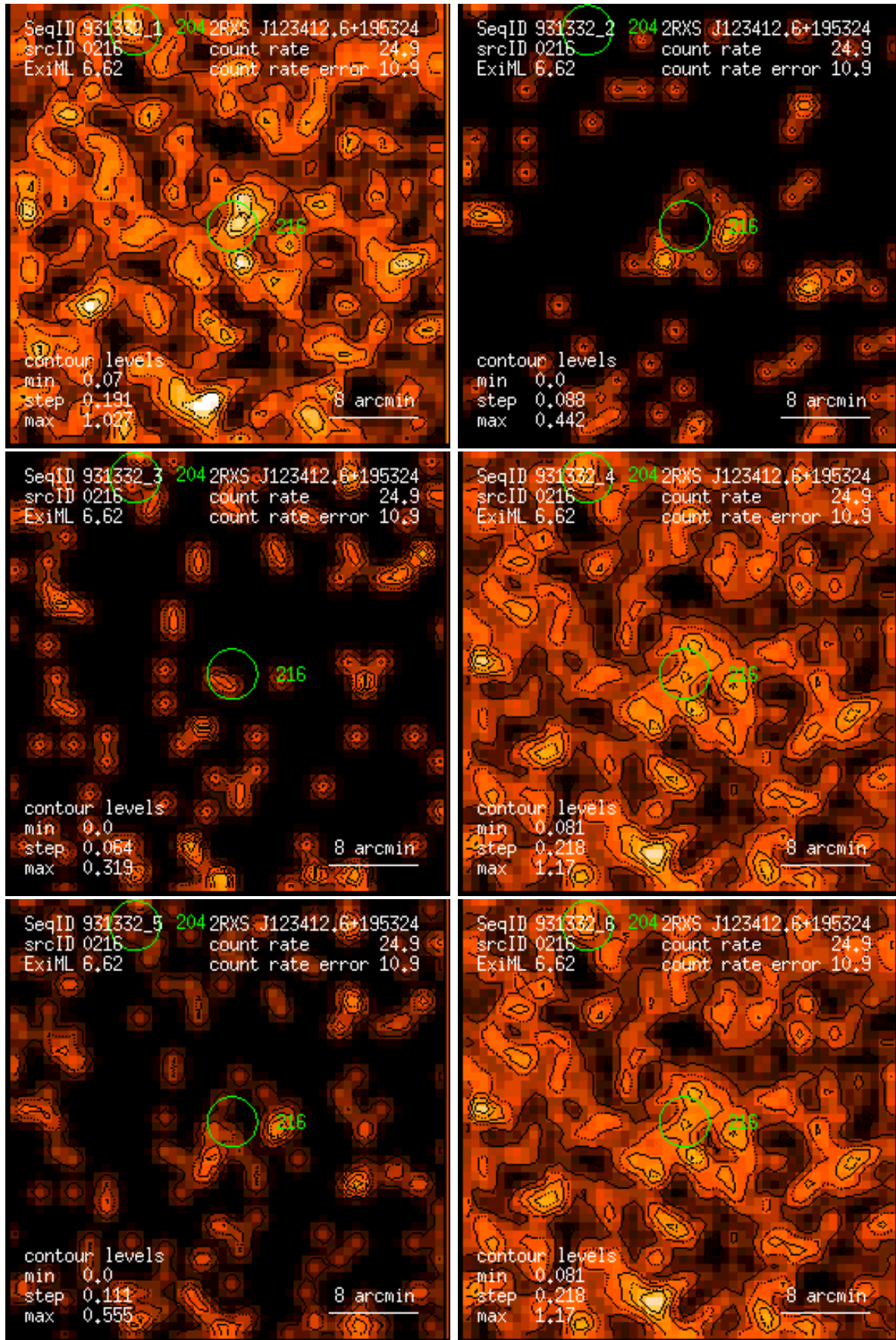
Figure 216: RASS 931332: detection 0216: band rate images, Gaussian filter: (1) PSPC channels 11 – 41, (2) 52 – 90, (3) 91 – 201, (4) 11 – 235, (5) 52 – 201, (6) 11 – 201. Broad band rates in counts/ks. Band rate contour levels in counts/ks/arcmin 2 .
