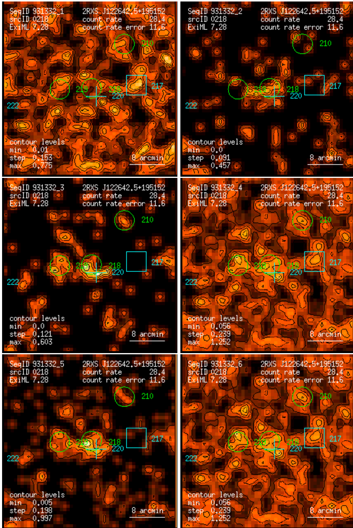
Figure 218: RASS 931332: detection 0218: band rate images, Gaussian filter: (1) PSPC channels 11 – 41, (2) 52 – 90, (3) 91 – 201, (4) 11 – 235, (5) 52 – 201, (6) 11 – 201. Broad band rates in counts/ks. Band rate contour levels in counts/ks/arcmin 2 .
