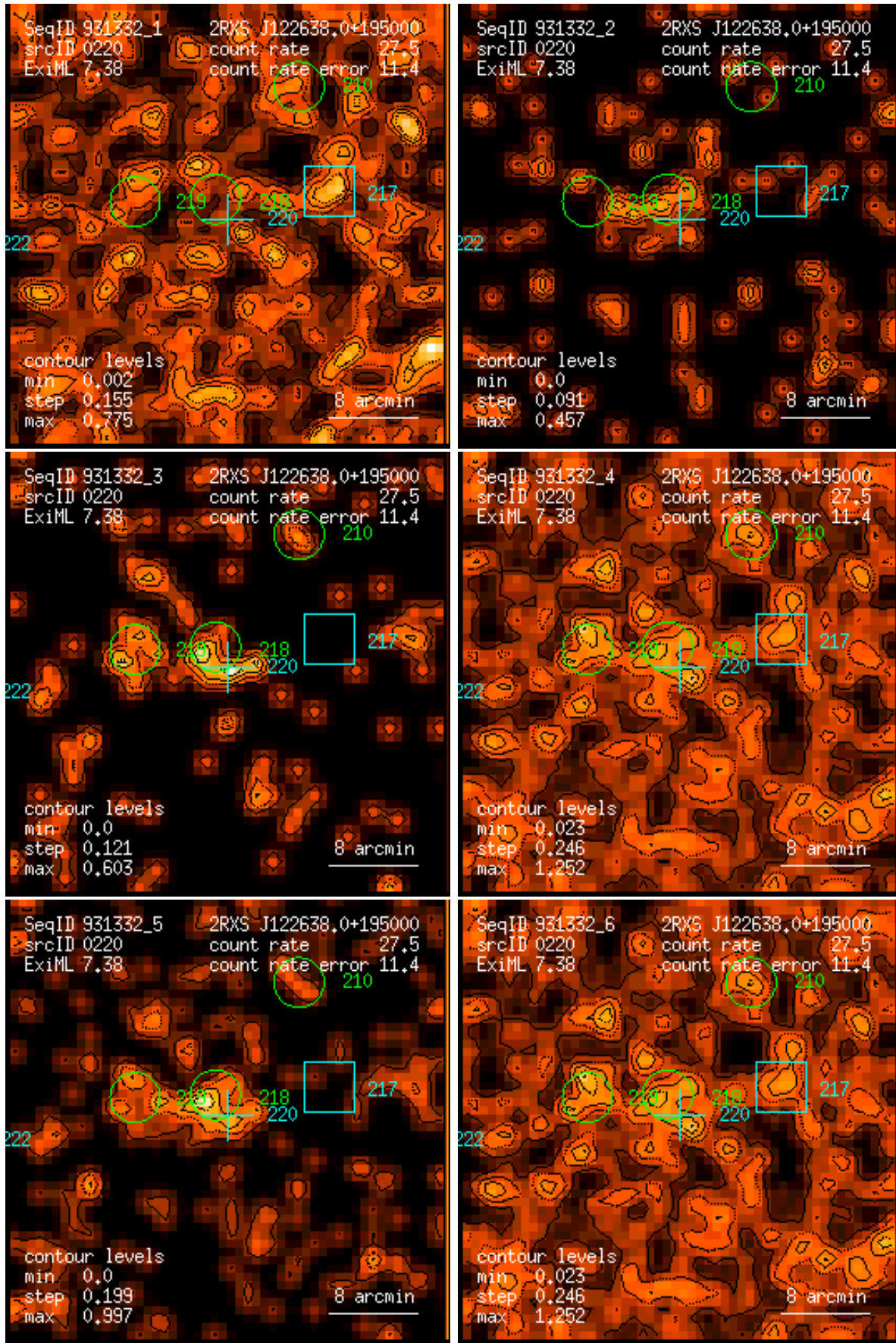
Figure 220: RASS 931332: detection 0220: band rate images, Gaussian filter: (1) PSPC channels 11 – 41, (2) 52 – 90, (3) 91 – 201, (4) 11 – 235, (5) 52 – 201, (6) 11 – 201. Broad band rates in counts/ks. Band rate contour levels in counts/ks/arcmin 2 .
