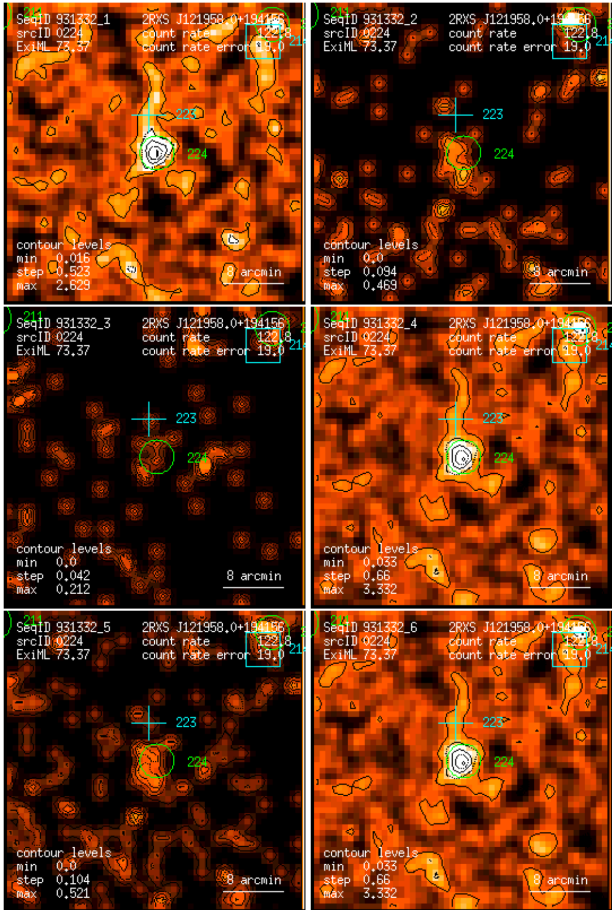
Figure 224: RASS 931332: detection 0224: band rate images, Gaussian filter: (1) PSPC channels 11 – 41, (2) 52 – 90, (3) 91 – 201, (4) 11 – 235, (5) 52 – 201, (6) 11 – 201. Broad band rates in counts/ks. Band rate contour levels in counts/ks/arcmin 2 .
