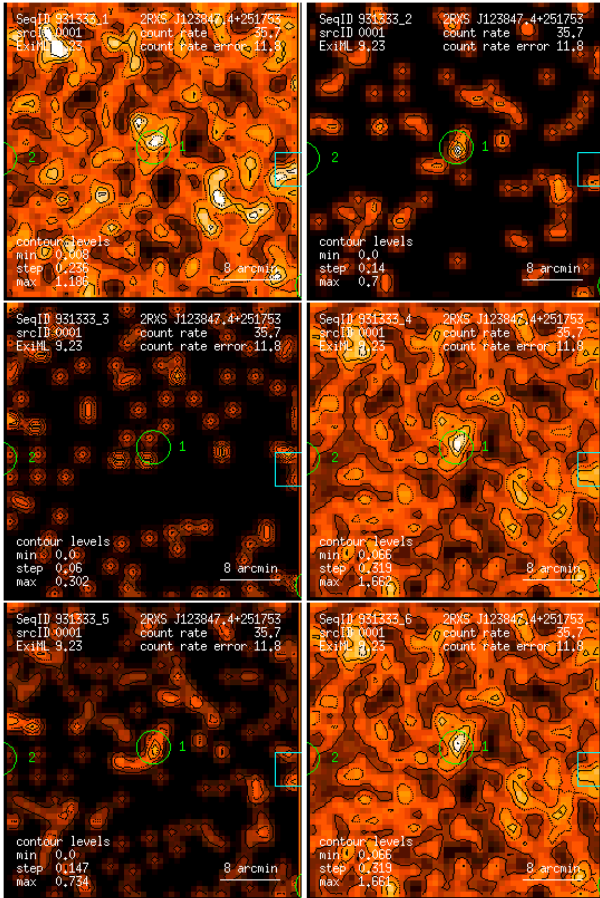
Figure 1: RASS 931333: detection 0001: band rate images, Gaussian filter: (1) PSPC channels 11 – 41, (2) 52 – 90, (3) 91 – 201, (4) 11 – 235, (5) 52 – 201, (6) 11 – 201. Broad band rates in counts/ks. Band rate contour levels in counts/ks/arcmin 2 .
