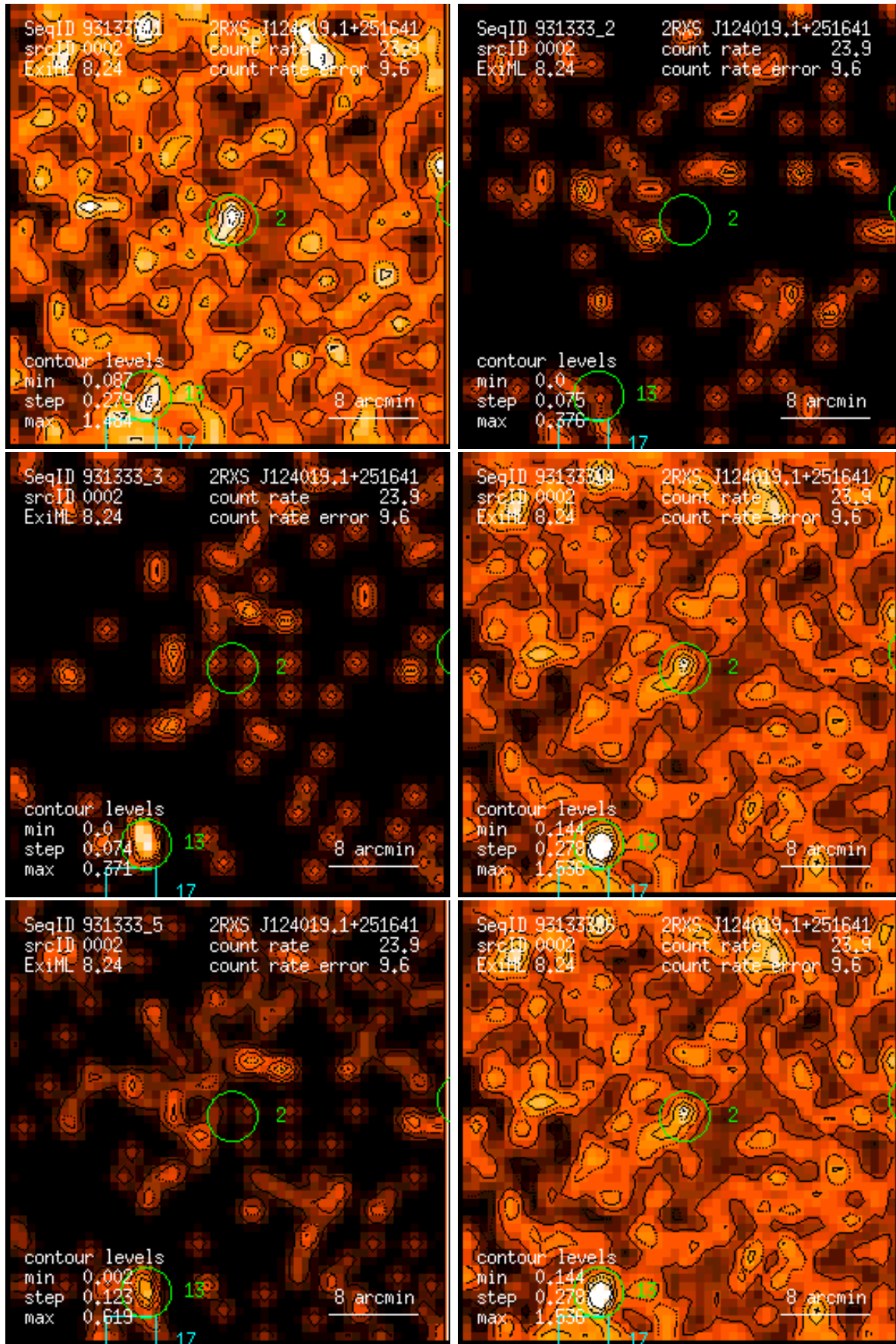
Figure 2: RASS 931333: detection 0002: band rate images, Gaussian filter: (1) PSPC channels 11 – 41, (2) 52 – 90, (3) 91 – 201, (4) 11 – 235, (5) 52 – 201, (6) 11 – 201. Broad band rates in counts/ks. Band rate contour levels in counts/ks/arcmin 2 .
