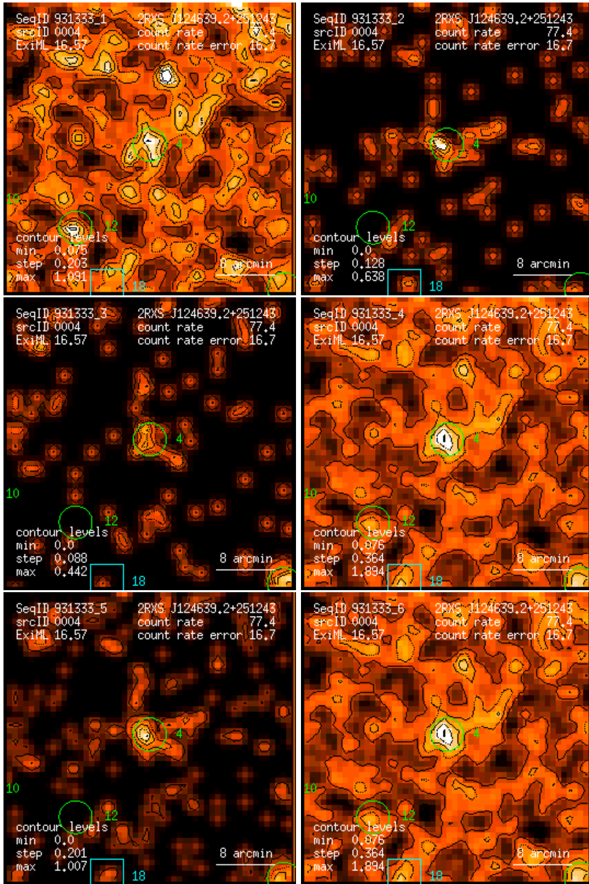
Figure 4: RASS 931333: detection 0004: band rate images, Gaussian filter: (1) PSPC channels 11 – 41, (2) 52 – 90, (3) 91 – 201, (4) 11 – 235, (5) 52 – 201, (6) 11 – 201. Broad band rates in counts/ks. Band rate contour levels in counts/ks/arcmin 2 .
