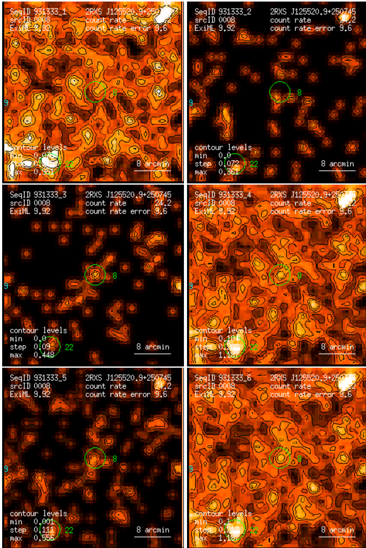
Figure 8: RASS 931333: detection 0008: band rate images, Gaussian filter: (1) PSPC channels 11 – 41, (2) 52 – 90, (3) 91 – 201, (4) 11 – 235, (5) 52 – 201, (6) 11 – 201. Broad band rates in counts/ks. Band rate contour levels in counts/ks/arcmin 2 .
