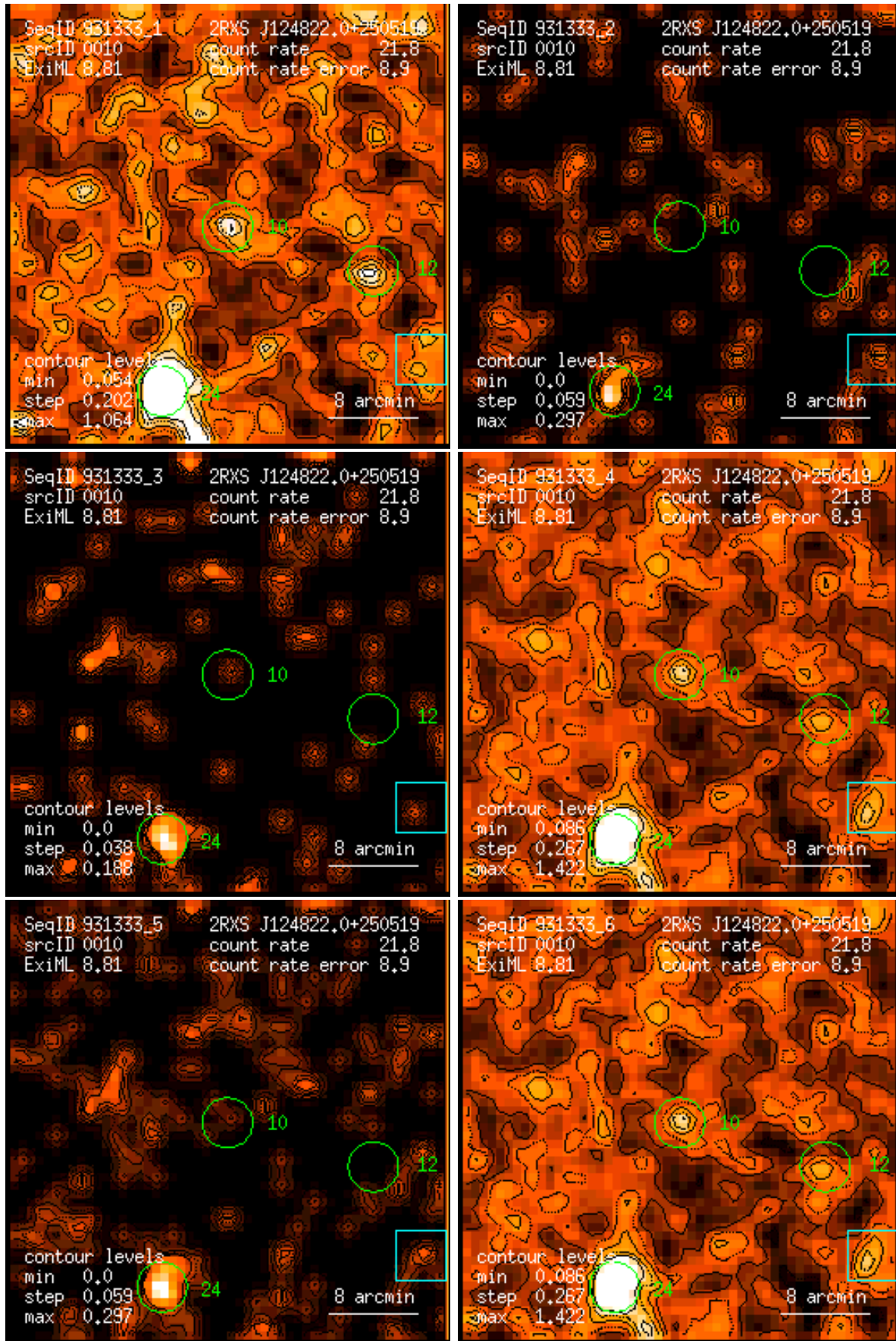
Figure 10: RASS 931333: detection 0010: band rate images, Gaussian filter: (1) PSPC channels 11 – 41, (2) 52 – 90, (3) 91 – 201, (4) 11 – 235, (5) 52 – 201, (6) 11 – 201. Broad band rates in counts/ks. Band rate contour levels in counts/ks/arcmin 2 .
