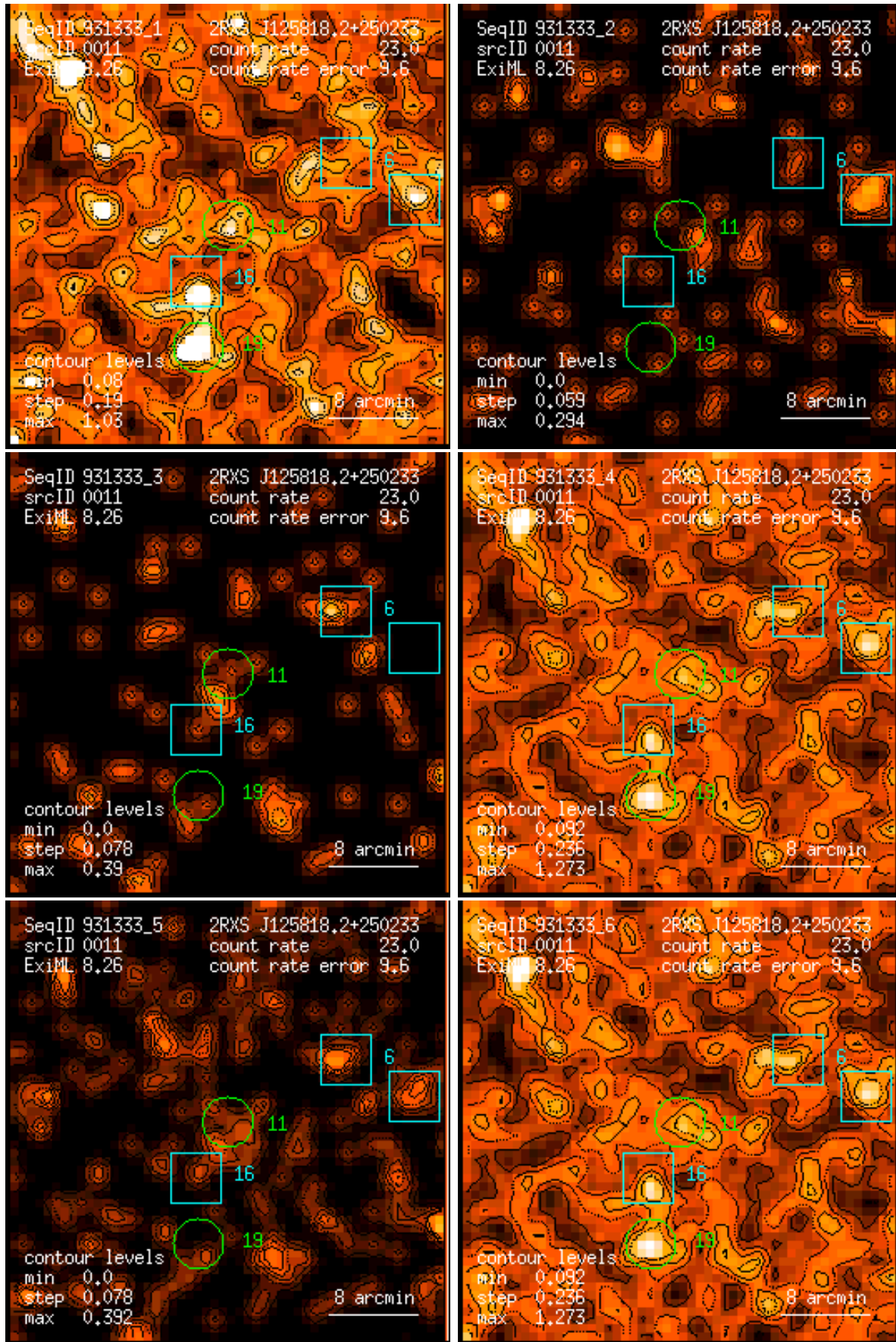
Figure 11: RASS 931333: detection 0011: band rate images, Gaussian filter: (1) PSPC channels 11 – 41, (2) 52 – 90, (3) 91 – 201, (4) 11 – 235, (5) 52 – 201, (6) 11 – 201. Broad band rates in counts/ks. Band rate contour levels in counts/ks/arcmin 2 .
