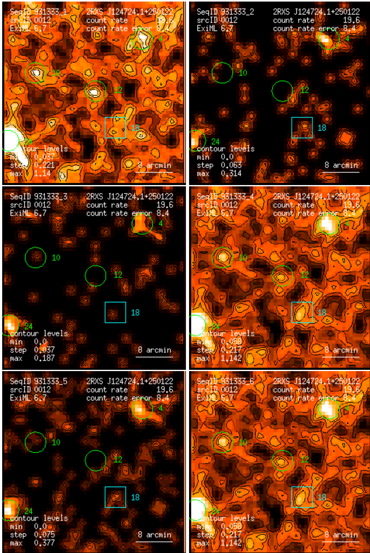
Figure 12: RASS 931333: detection 0012: band rate images, Gaussian filter: (1) PSPC channels 11 – 41, (2) 52 – 90, (3) 91 – 201, (4) 11 – 235, (5) 52 – 201, (6) 11 – 201. Broad band rates in counts/ks. Band rate contour levels in counts/ks/arcmin 2 .
