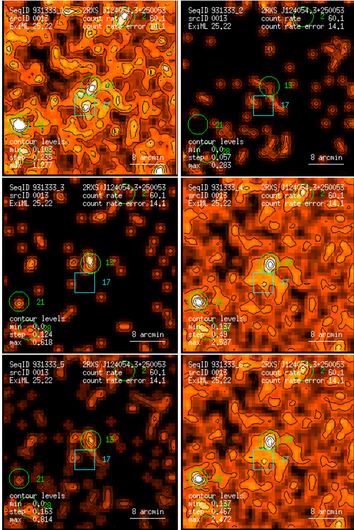
Figure 13: RASS 931333: detection 0013: band rate images, Gaussian filter: (1) PSPC channels 11 – 41, (2) 52 – 90, (3) 91 – 201, (4) 11 – 235, (5) 52 – 201, (6) 11 – 201. Broad band rates in counts/ks. Band rate contour levels in counts/ks/arcmin 2 .
