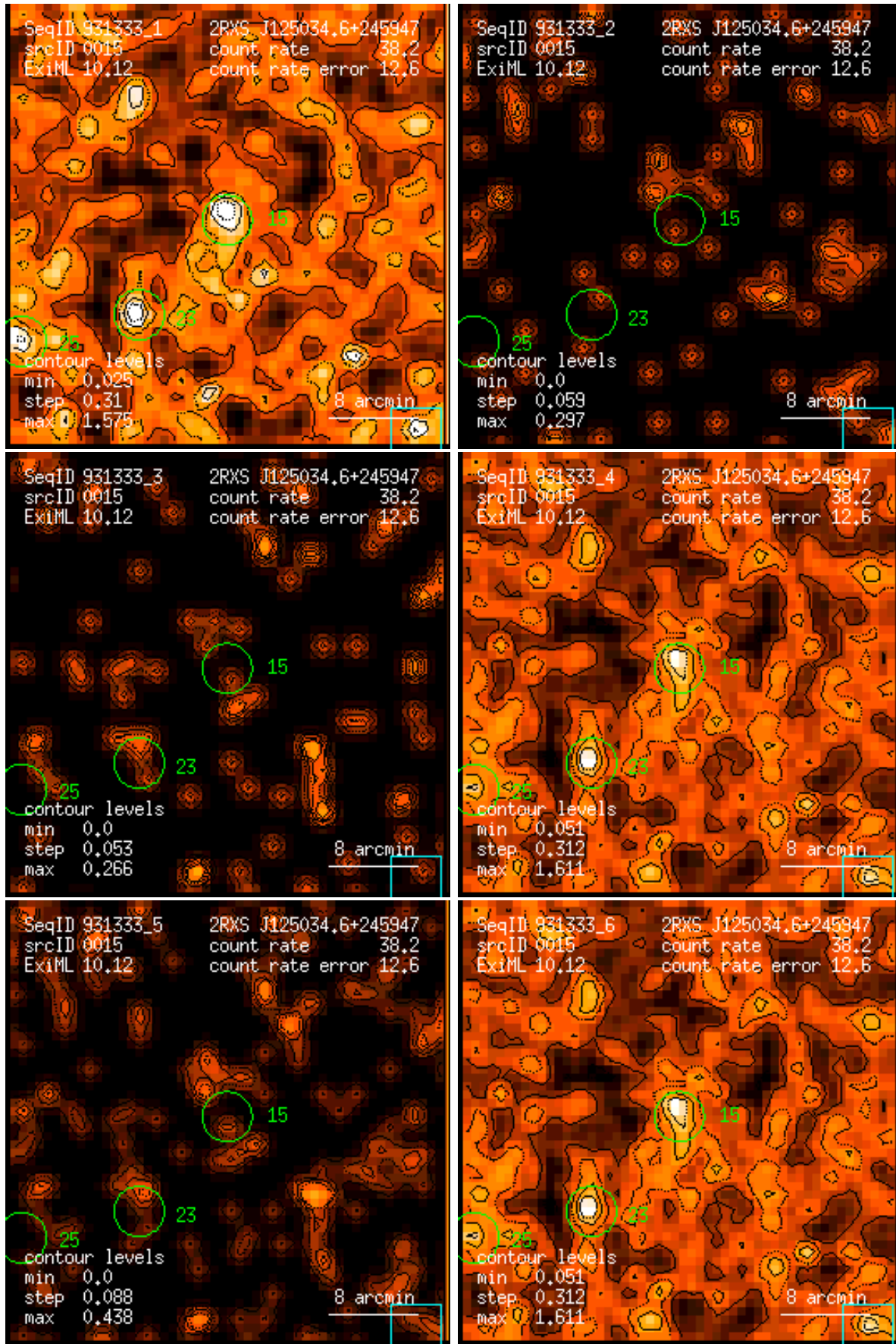
Figure 15: RASS 931333: detection 0015: band rate images, Gaussian filter: (1) PSPC channels 11 – 41, (2) 52 – 90, (3) 91 – 201, (4) 11 – 235, (5) 52 – 201, (6) 11 – 201. Broad band rates in counts/ks. Band rate contour levels in counts/ks/arcmin 2 .
