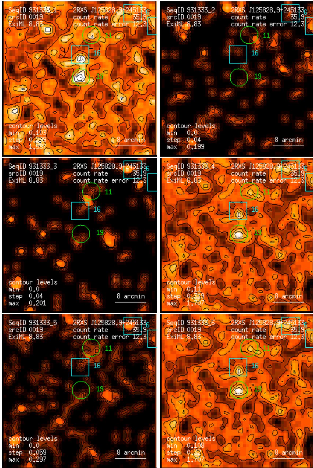
Figure 19: RASS 931333: detection 0019: band rate images, Gaussian filter: (1) PSPC channels 11 – 41, (2) 52 – 90, (3) 91 – 201, (4) 11 – 235, (5) 52 – 201, (6) 11 – 201. Broad band rates in counts/ks. Band rate contour levels in counts/ks/arcmin 2 .
