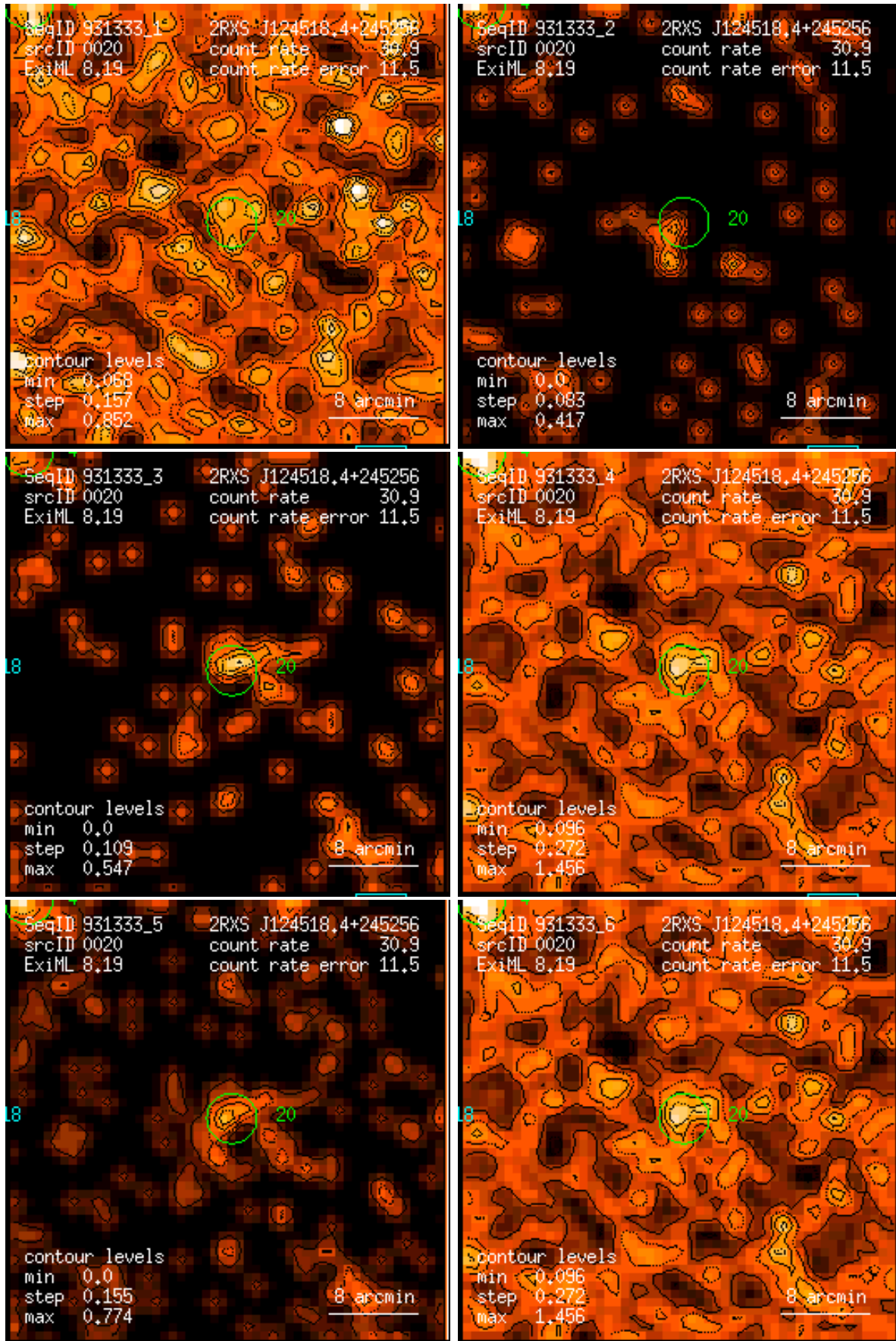
Figure 20: RASS 931333: detection 0020: band rate images, Gaussian filter: (1) PSPC channels 11 – 41, (2) 52 – 90, (3) 91 – 201, (4) 11 – 235, (5) 52 – 201, (6) 11 – 201. Broad band rates in counts/ks. Band rate contour levels in counts/ks/arcmin 2 .
