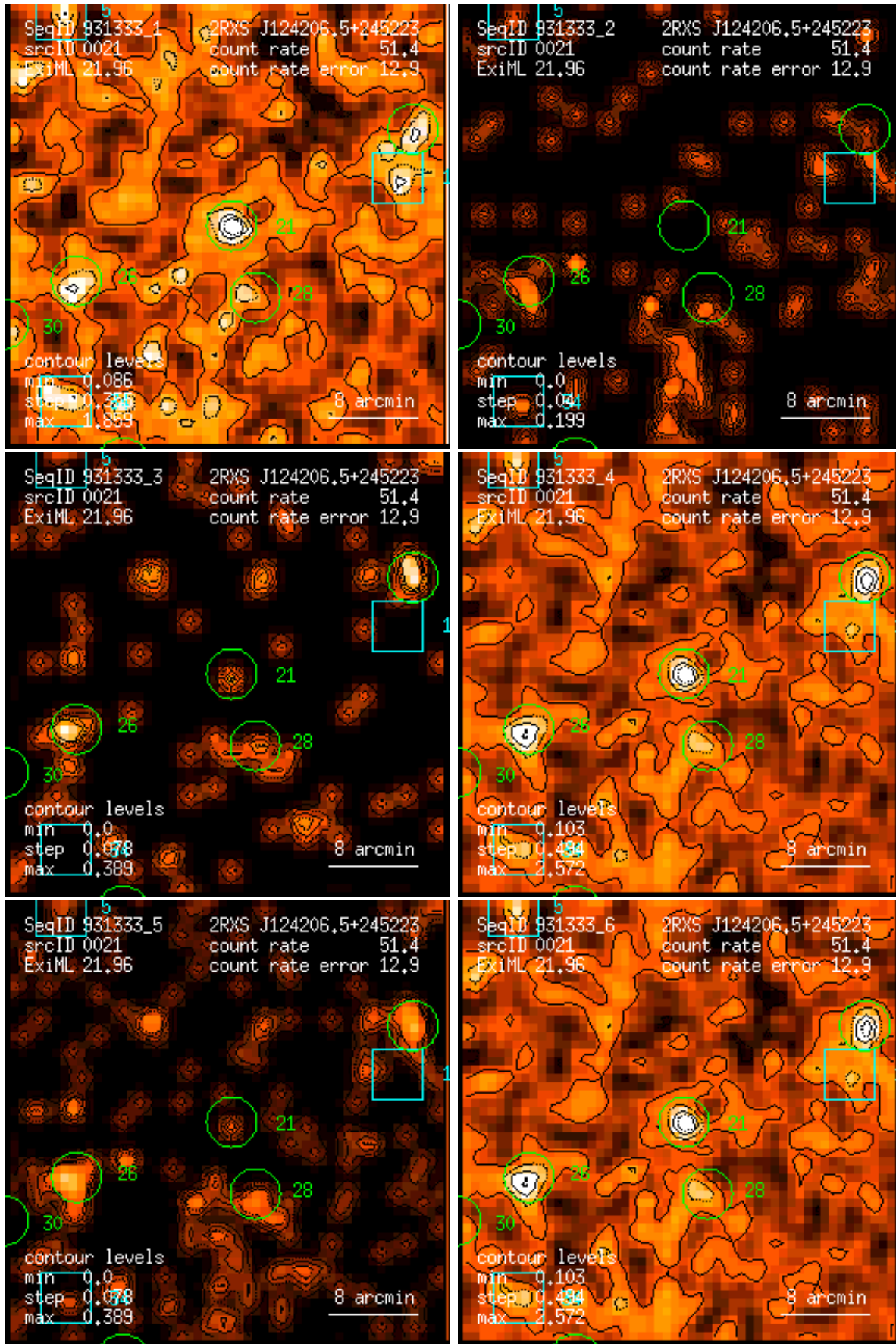
Figure 21: RASS 931333: detection 0021: band rate images, Gaussian filter: (1) PSPC channels 11 – 41, (2) 52 – 90, (3) 91 – 201, (4) 11 – 235, (5) 52 – 201, (6) 11 – 201. Broad band rates in counts/ks. Band rate contour levels in counts/ks/arcmin 2 .
