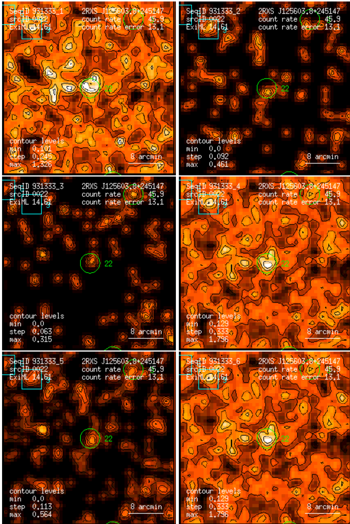
Figure 22: RASS 931333: detection 0022: band rate images, Gaussian filter: (1) PSPC channels 11 – 41, (2) 52 – 90, (3) 91 – 201, (4) 11 – 235, (5) 52 – 201, (6) 11 – 201. Broad band rates in counts/ks. Band rate contour levels in counts/ks/arcmin 2 .
