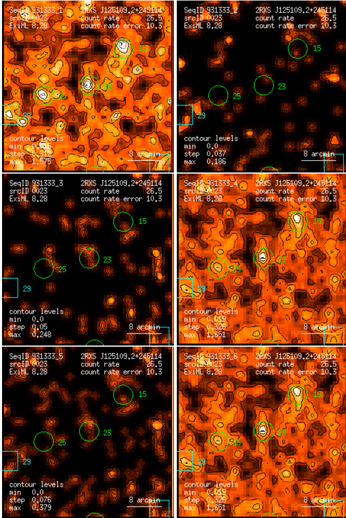
Figure 23: RASS 931333: detection 0023: band rate images, Gaussian filter: (1) PSPC channels 11 – 41, (2) 52 – 90, (3) 91 – 201, (4) 11 – 235, (5) 52 – 201, (6) 11 – 201. Broad band rates in counts/ks. Band rate contour levels in counts/ks/arcmin 2 .
