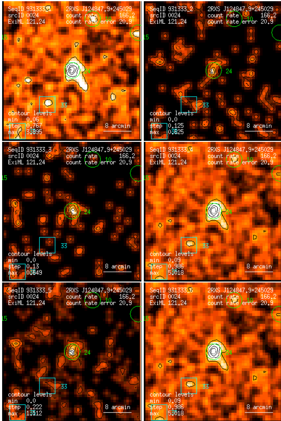
Figure 24: RASS 931333: detection 0024: band rate images, Gaussian filter: (1) PSPC channels 11 – 41, (2) 52 – 90, (3) 91 – 201, (4) 11 – 235, (5) 52 – 201, (6) 11 – 201. Broad band rates in counts/ks. Band rate contour levels in counts/ks/arcmin 2 .
