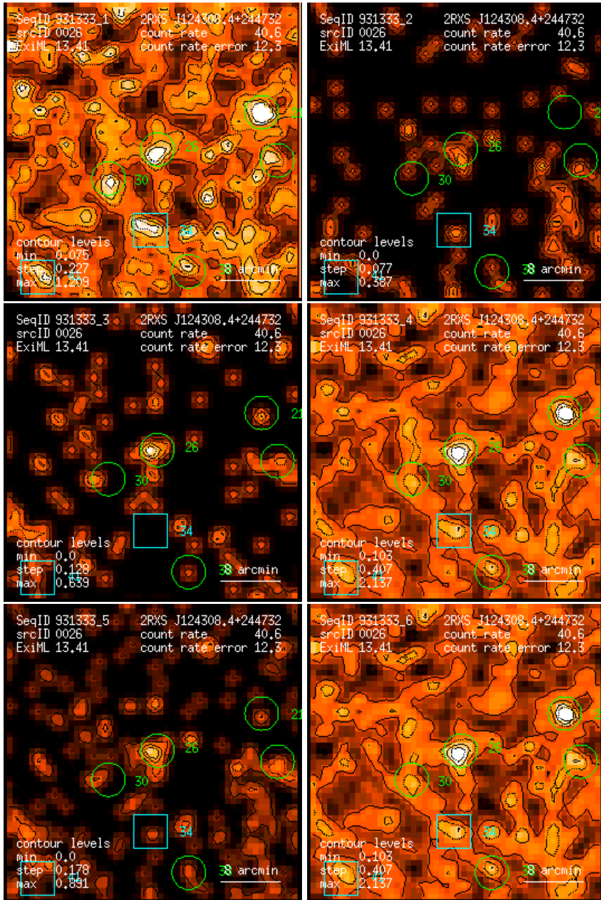
Figure 26: RASS 931333: detection 0026: band rate images, Gaussian filter: (1) PSPC channels 11 – 41, (2) 52 – 90, (3) 91 – 201, (4) 11 – 235, (5) 52 – 201, (6) 11 – 201. Broad band rates in counts/ks. Band rate contour levels in counts/ks/arcmin 2 .
