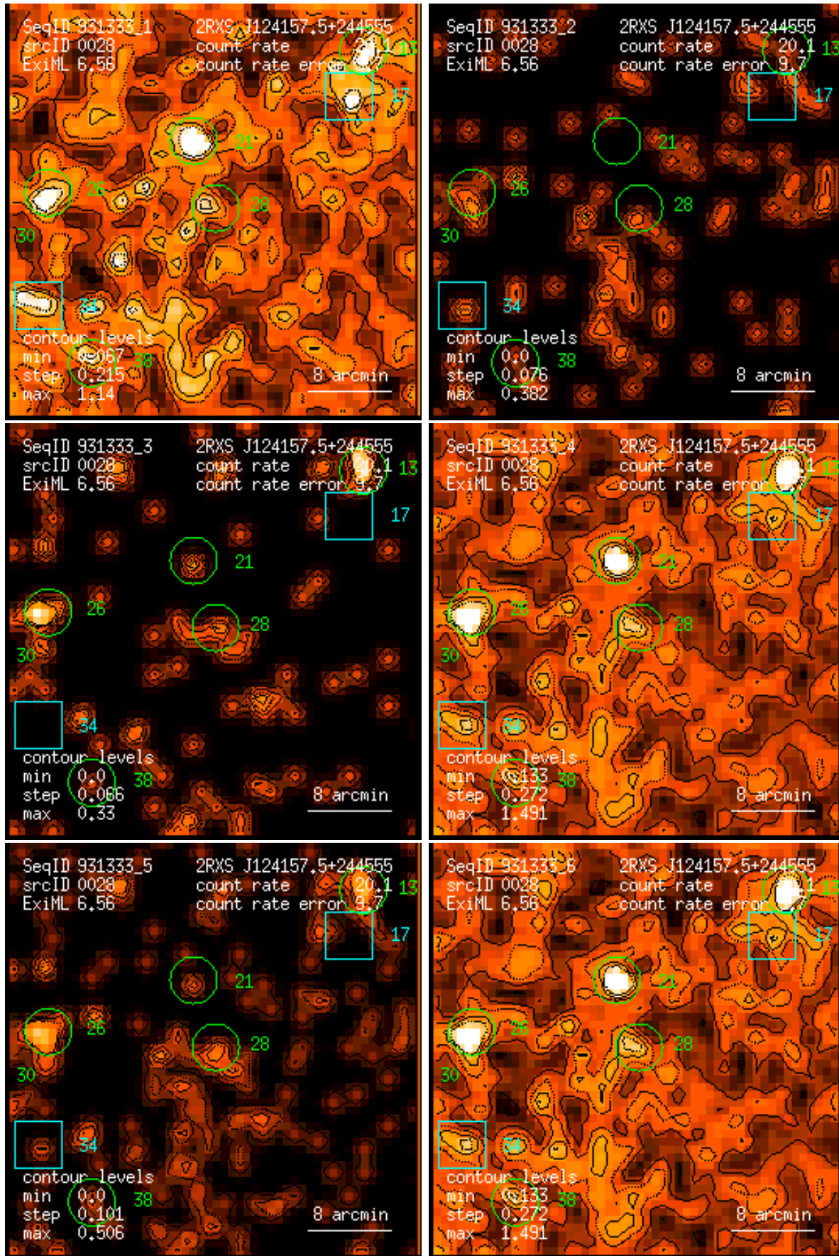
Figure 28: RASS 931333: detection 0028: band rate images, Gaussian filter: (1) PSPC channels 11 – 41, (2) 52 – 90, (3) 91 – 201, (4) 11 – 235, (5) 52 – 201, (6) 11 – 201. Broad band rates in counts/ks. Band rate contour levels in counts/ks/arcmin 2 .
